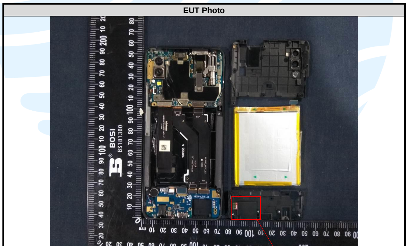
2/3/4G Antenna
