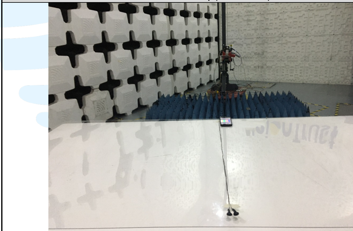
Radiated emission Test Setup (Above 1 GHz) - Mode 5
