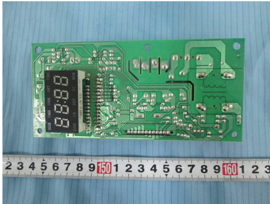
EUT – Control Panel Mainboard Bottom View
