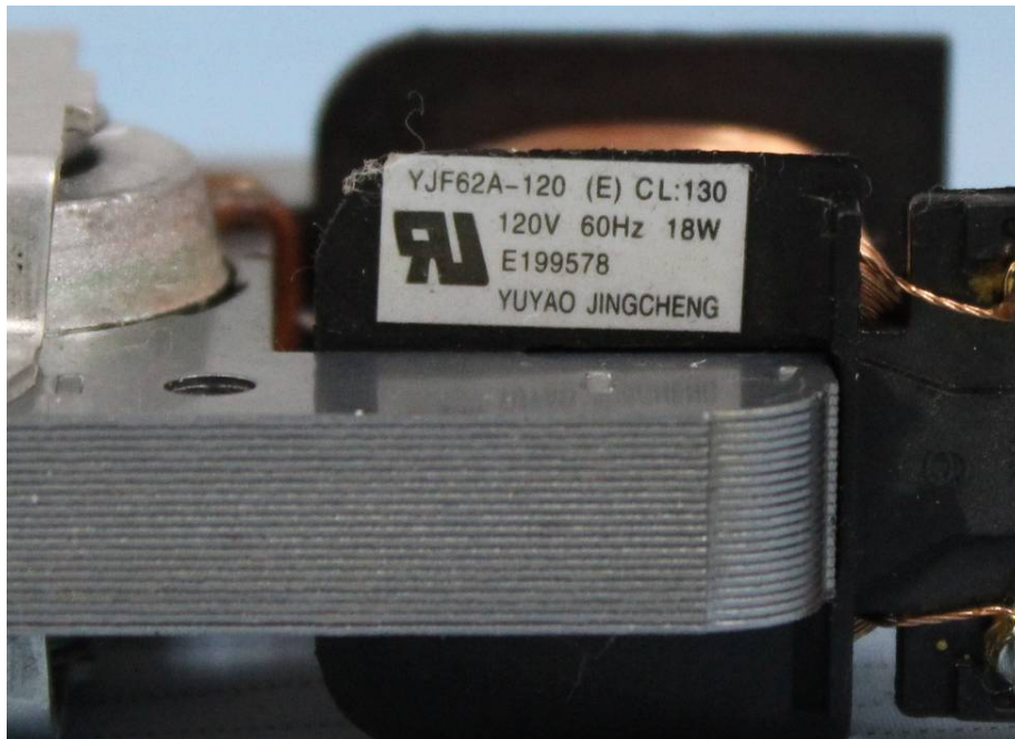
EUT –Fan Motor Label View
