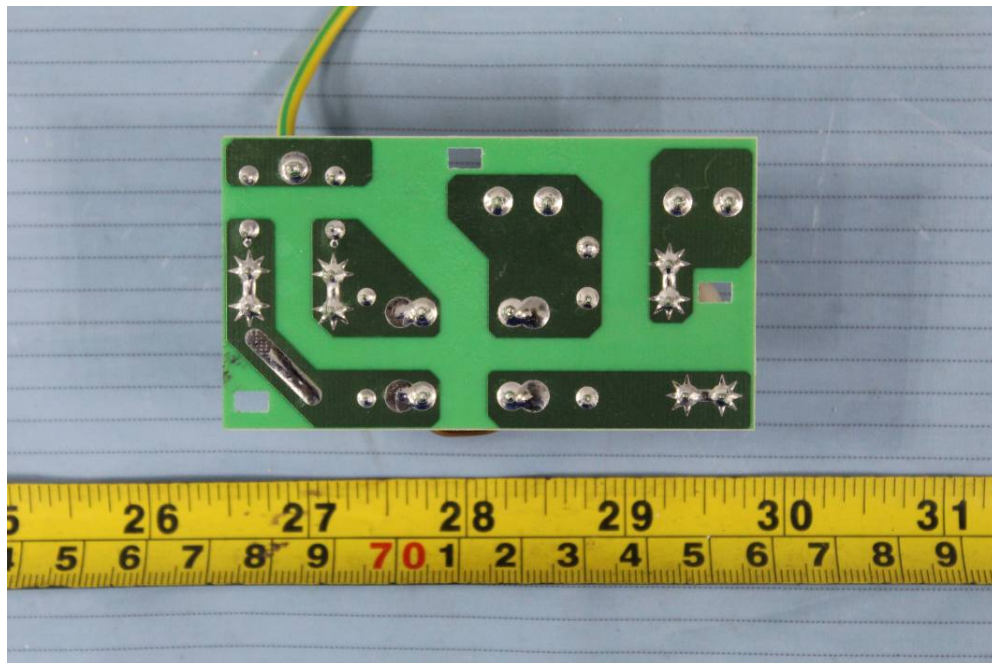
EUT –Power Board Bottom View
