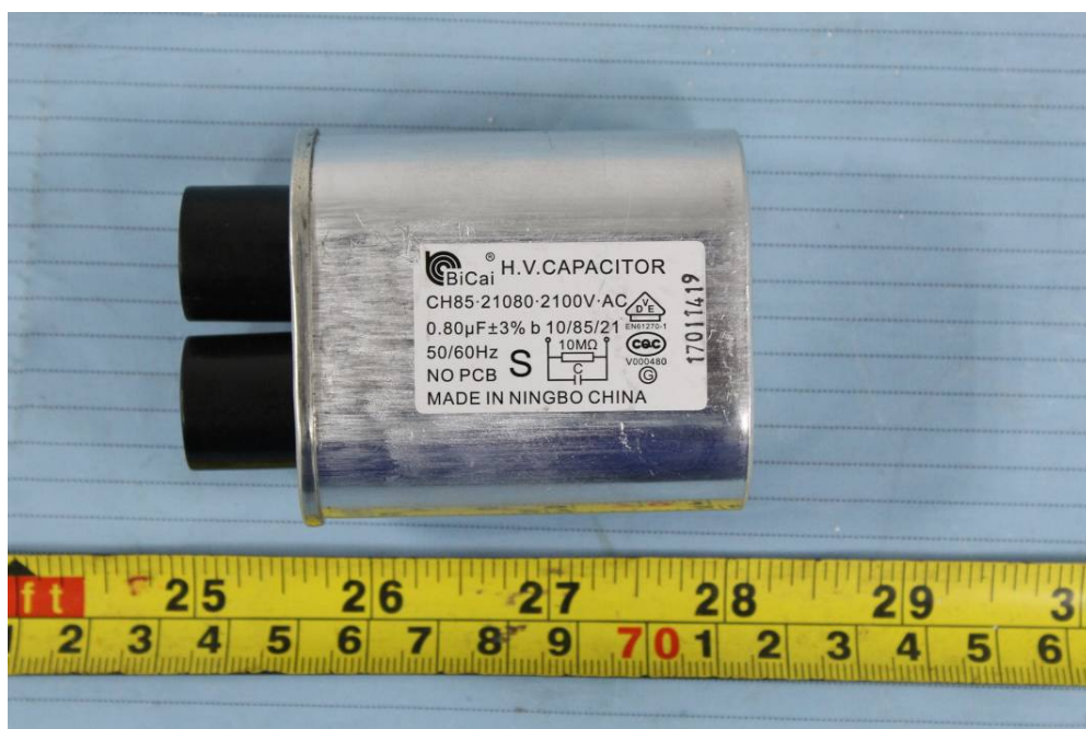
EUT – High Voltage Capacitor Label View
