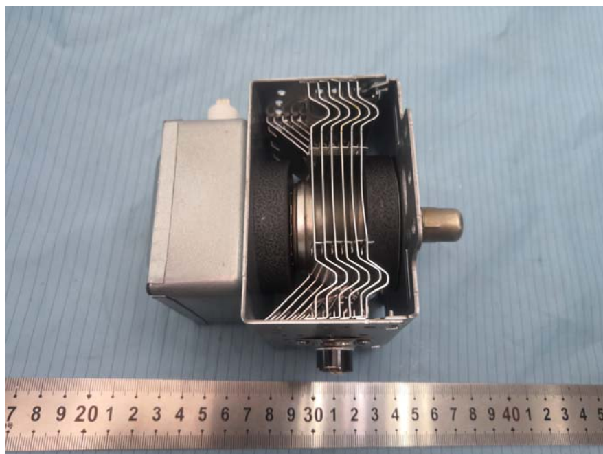
EUT – Magnetron Front View (Type 1)
