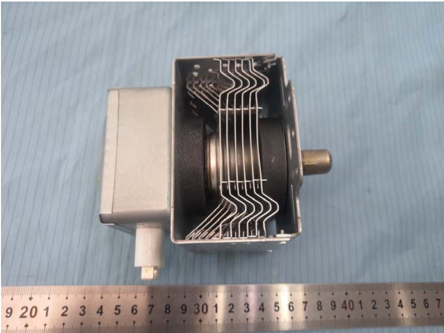
EUT – Magnetron Rear View (Type 1)
