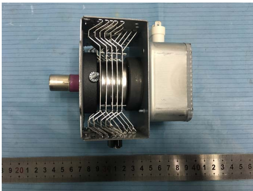
EUT – Magnetron Front View (Type 2)
