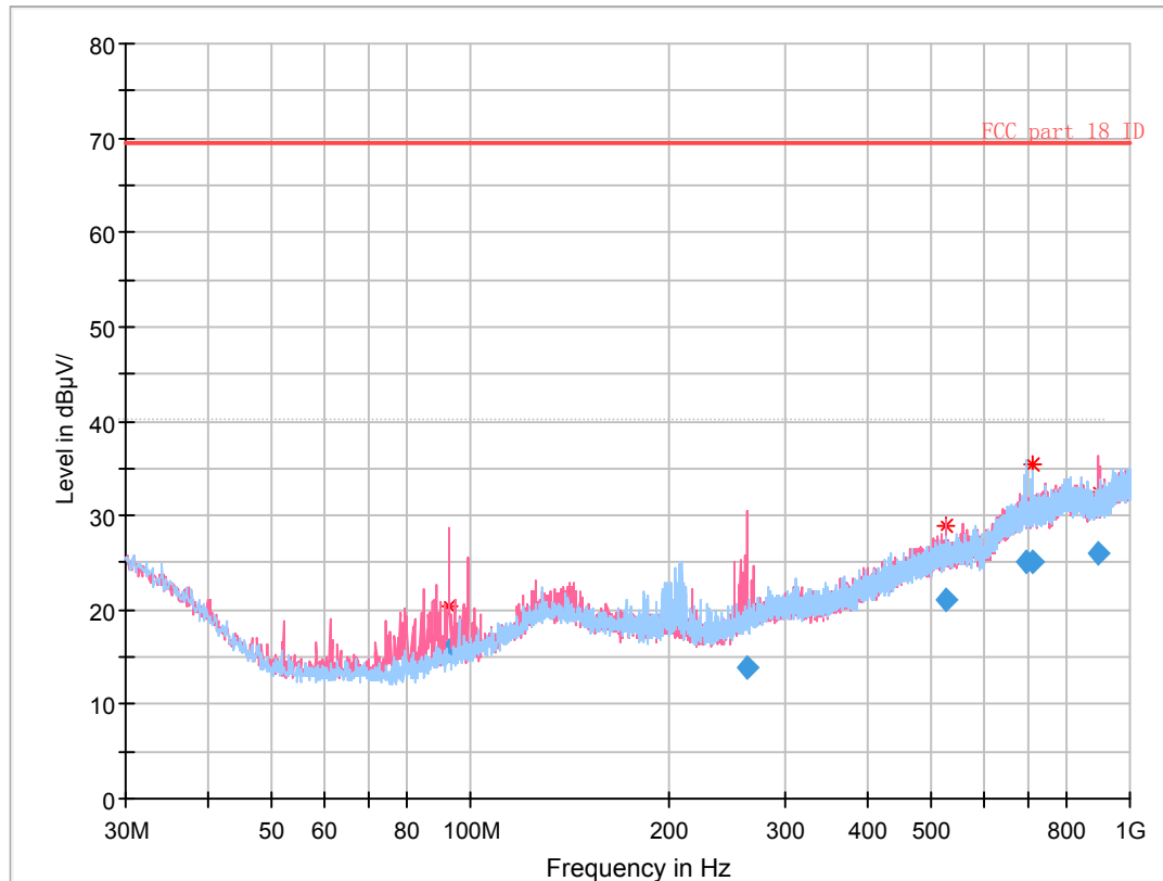
Full Spectrum
