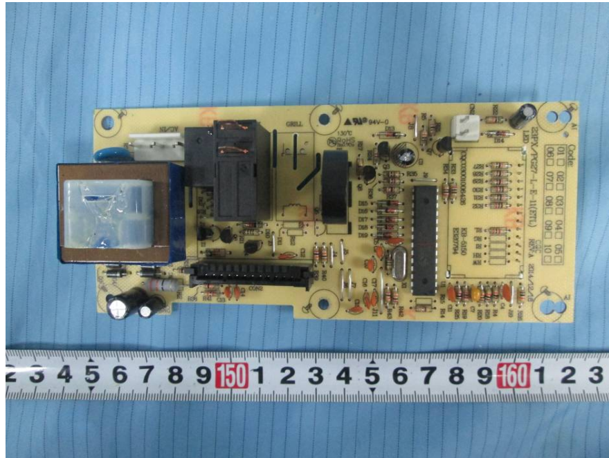
EUT –Control Panel Board Top View
