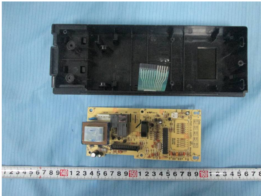
EUT –Control Panel Covered off View
