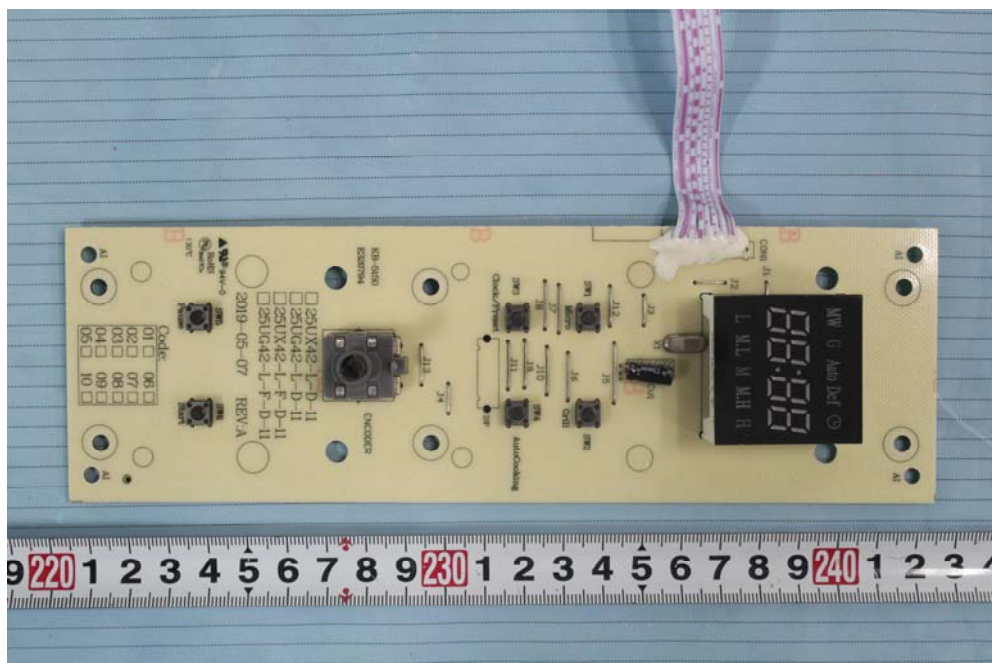
EUT – Control Board Top View
