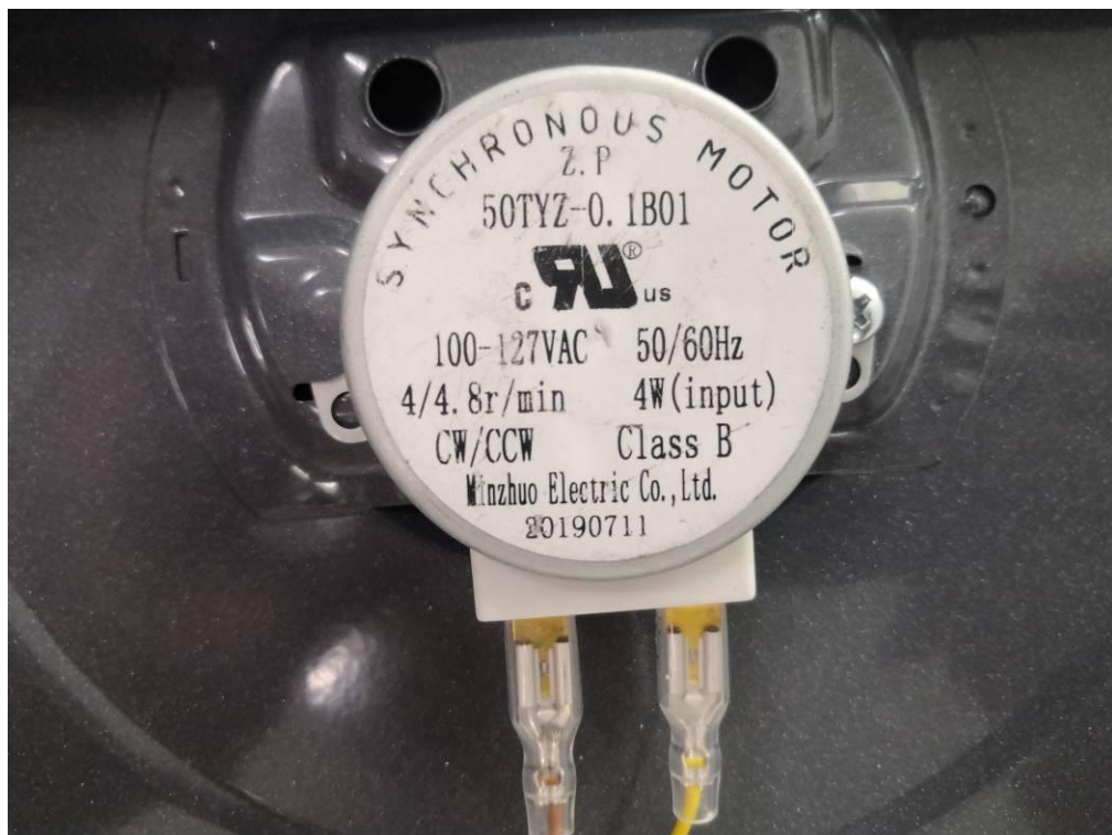
EUT – Motor View
