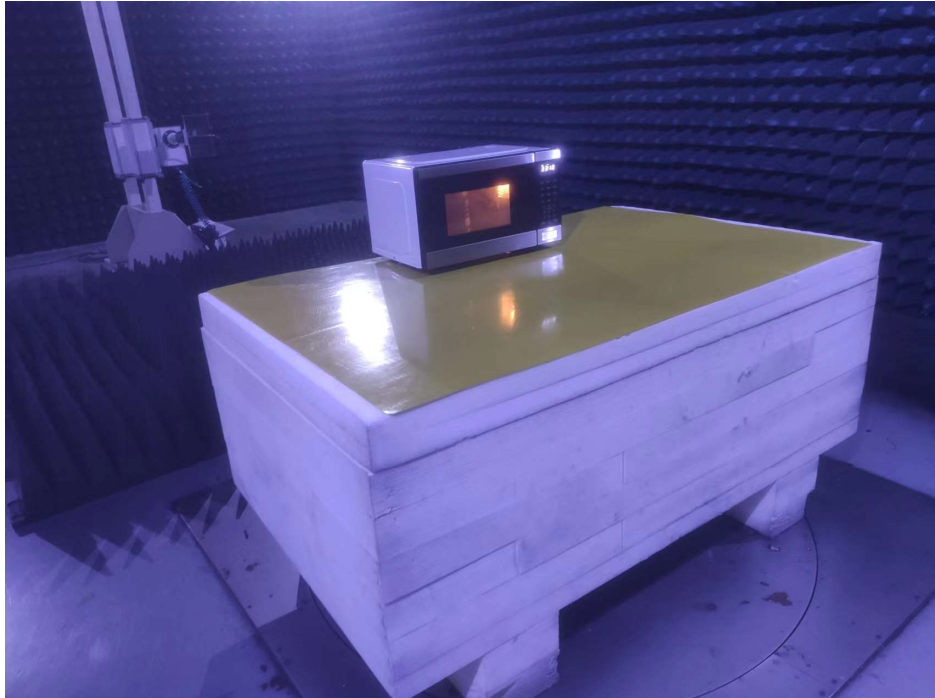
Photo of Radiation Emission Measurement- Above 1GHz
