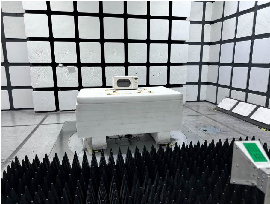
Radiated Emissions Front View (Above 18 GHz)
