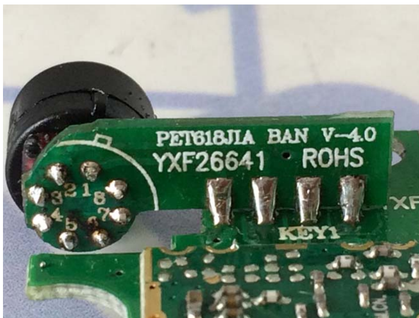
PCB 2 side 1
