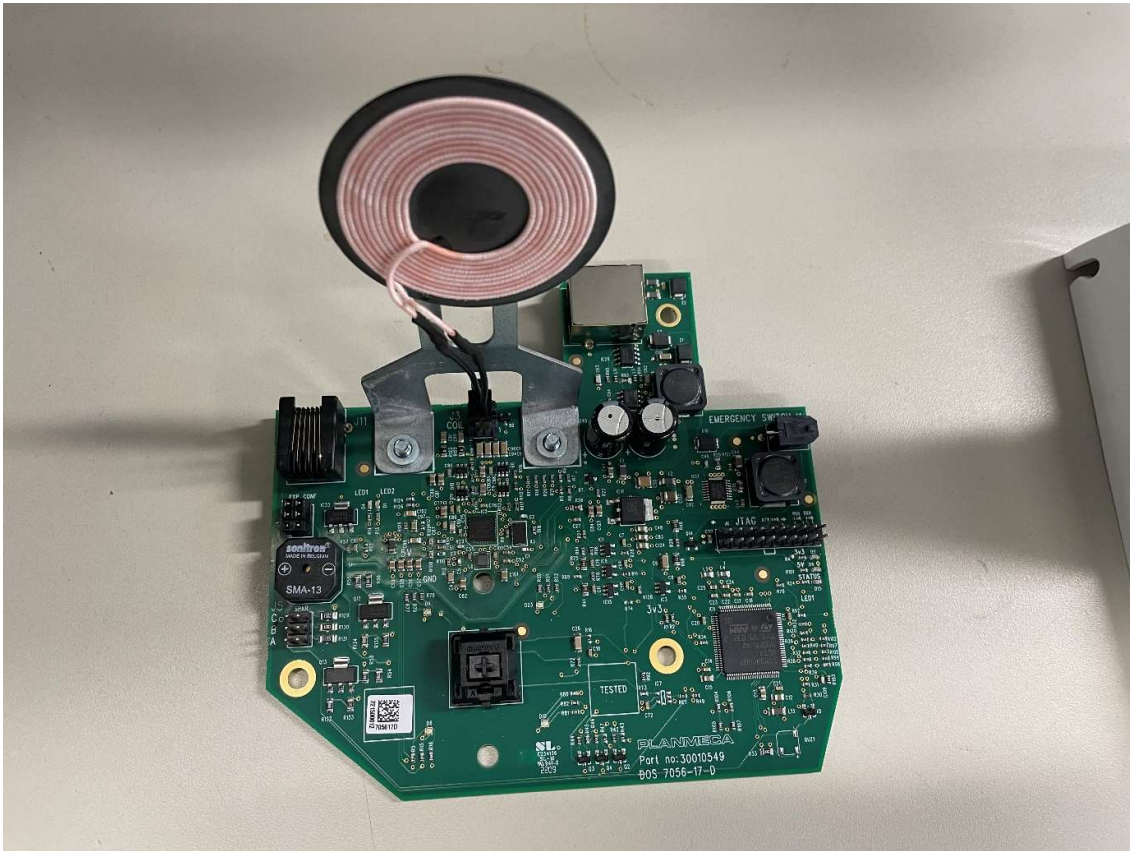
2. docking station PCB top
