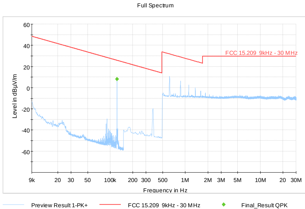
Figure 3: Radiated emission 9 kHz to 30MHz.
