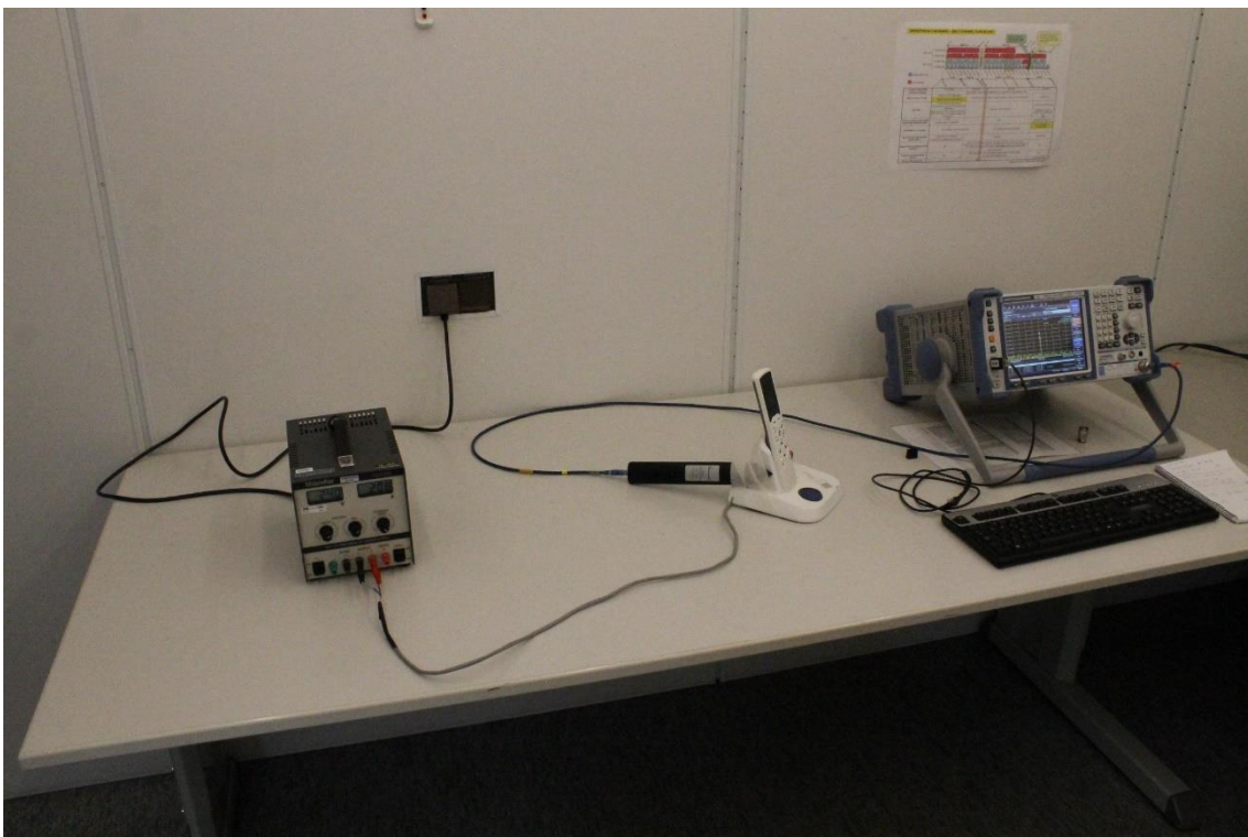
Photograph 4. 20 dB Emission Bandwidth
