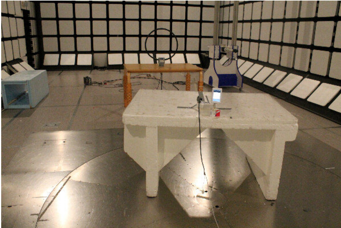
Photograph 1. Radiated emissions 0.009 - 30 MHz
