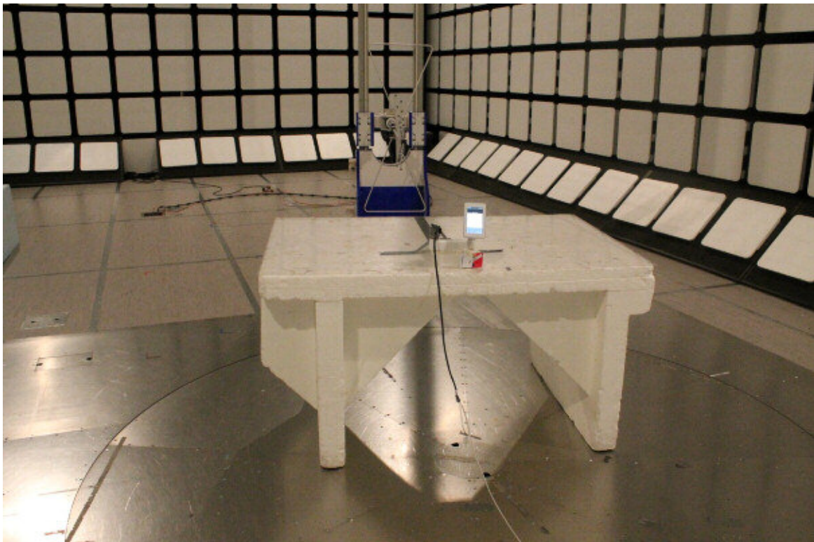
Photograph 2. Radiated emissions 30 - 1000 MHz
