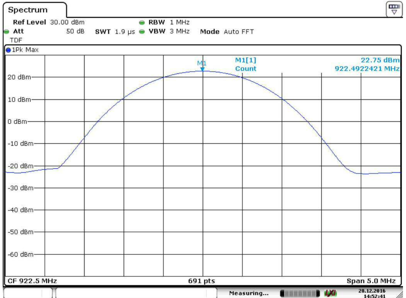
Figure 3. Channel HIGH.
