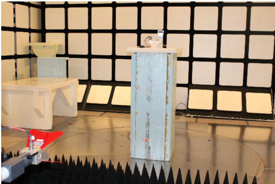
Photograph 3. Radiated emissions 1000 - 10000 MHz
