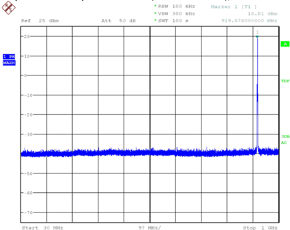
Graph 8: Conducted spurious emissions (non-restricted band), 30 MHz-1 GHz
