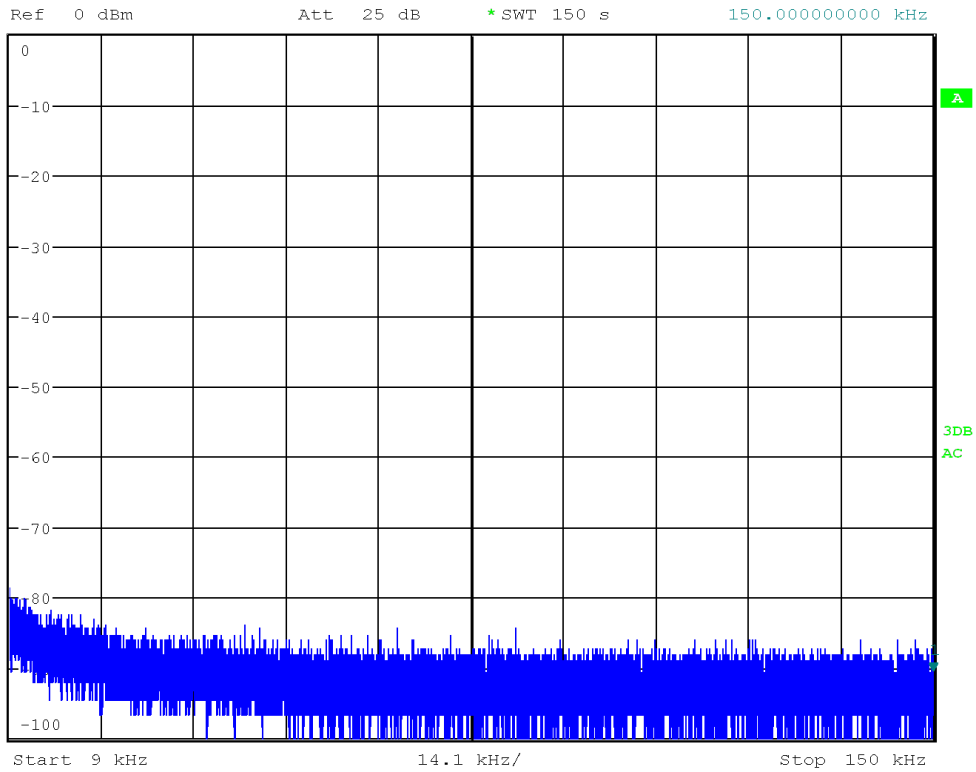
Conducted spurious emissions, 9 kHz-150 kHz
