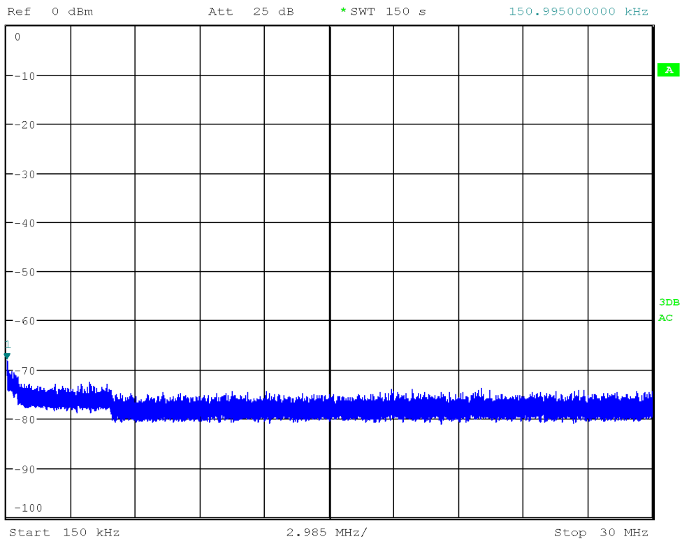
Conducted spurious emissions, 150 kHz-30 MHz
