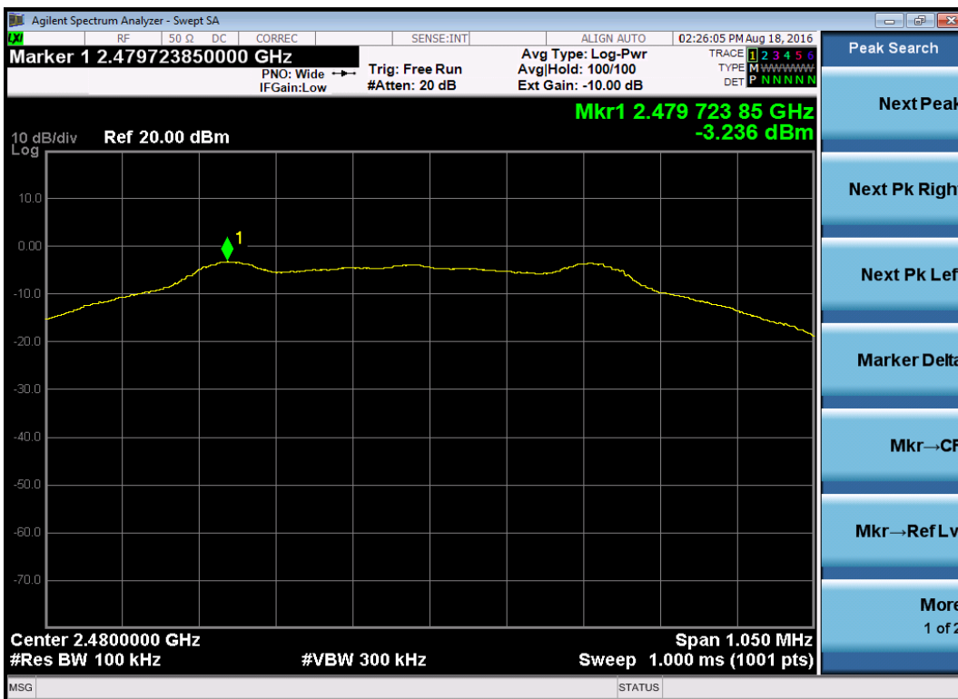
High Channel – Peak Power Spectral Density
