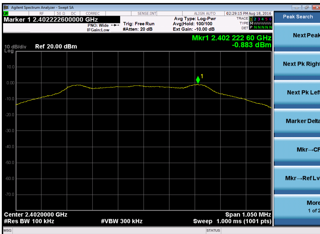
Low Channel – Peak Power Spectral Density
