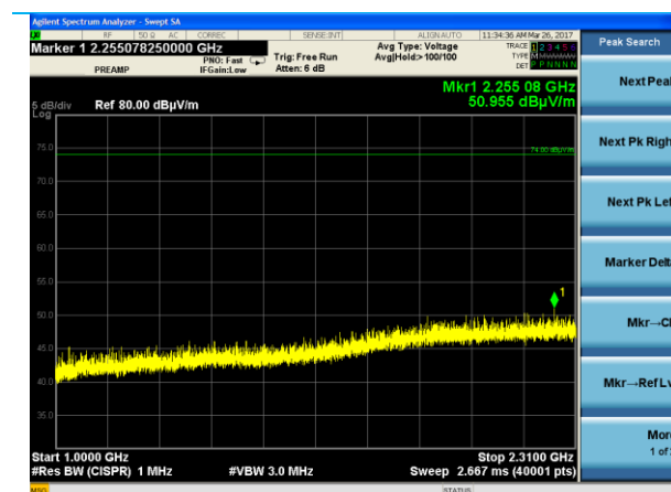
1000-2300 MHz (Peak)
