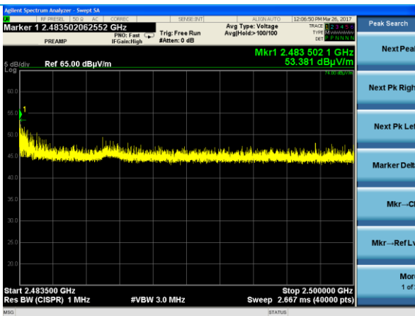
2483.5-2500 MHz (Peak)
