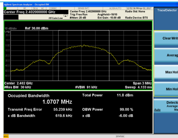
99% OBW
