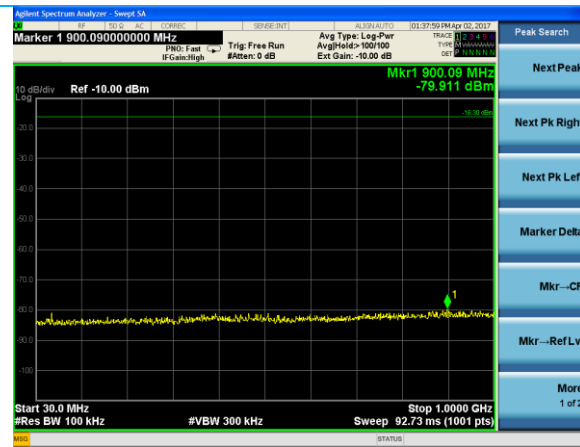
30 MHz – 1000 MHz
