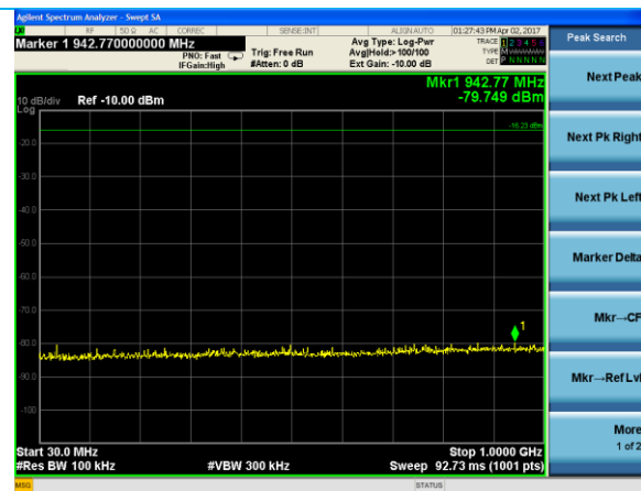
30 MHz - 1000 MHz
