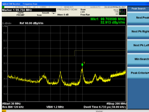
30-200 MHz Horizontal Polarity (EUT OFF)
