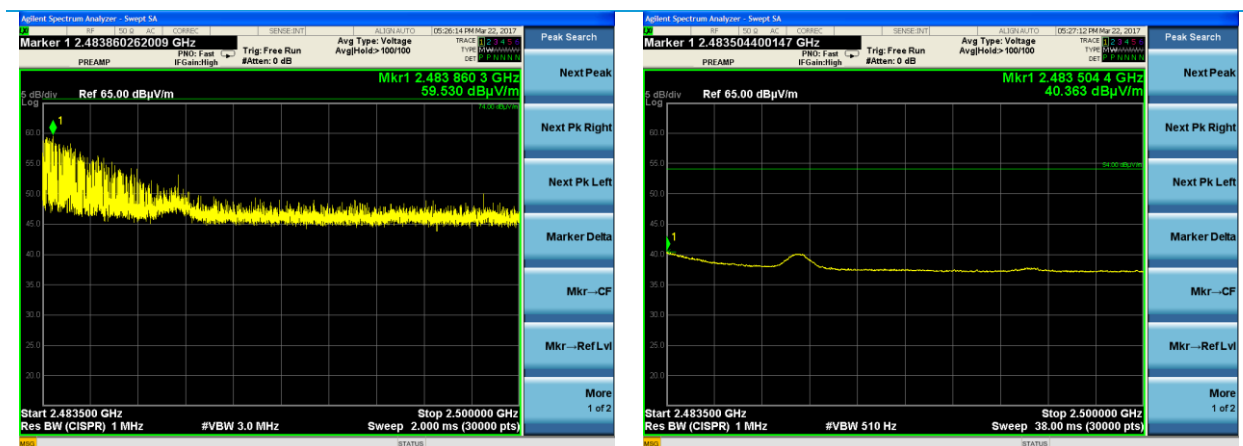
2483.5-2500 MHz (Peak)
