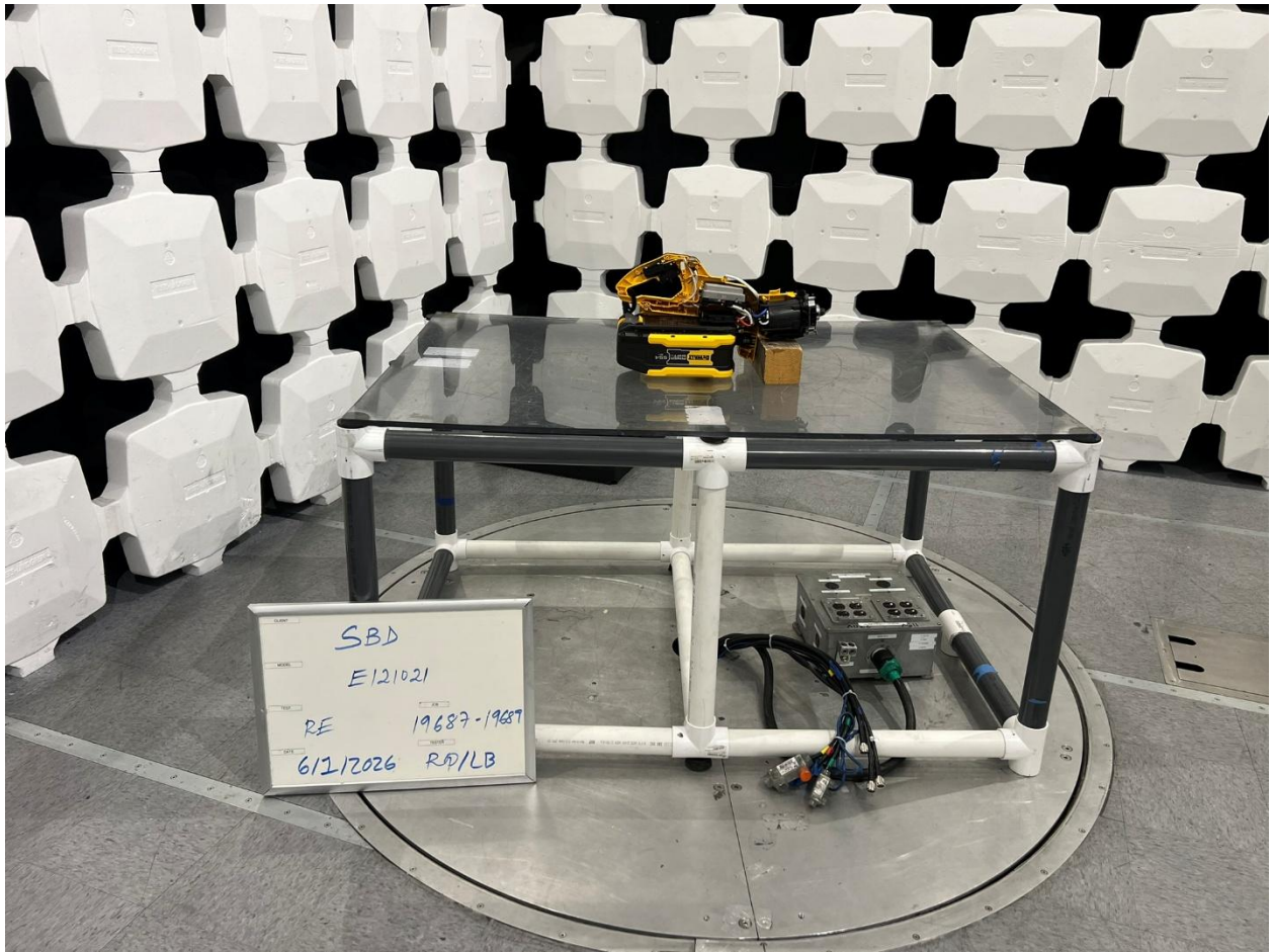
30MHz to 1GHz Radiated Emissions, View 3
