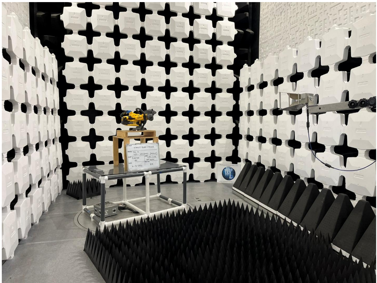
Above 1GHz Radiated Emissions, View 1
