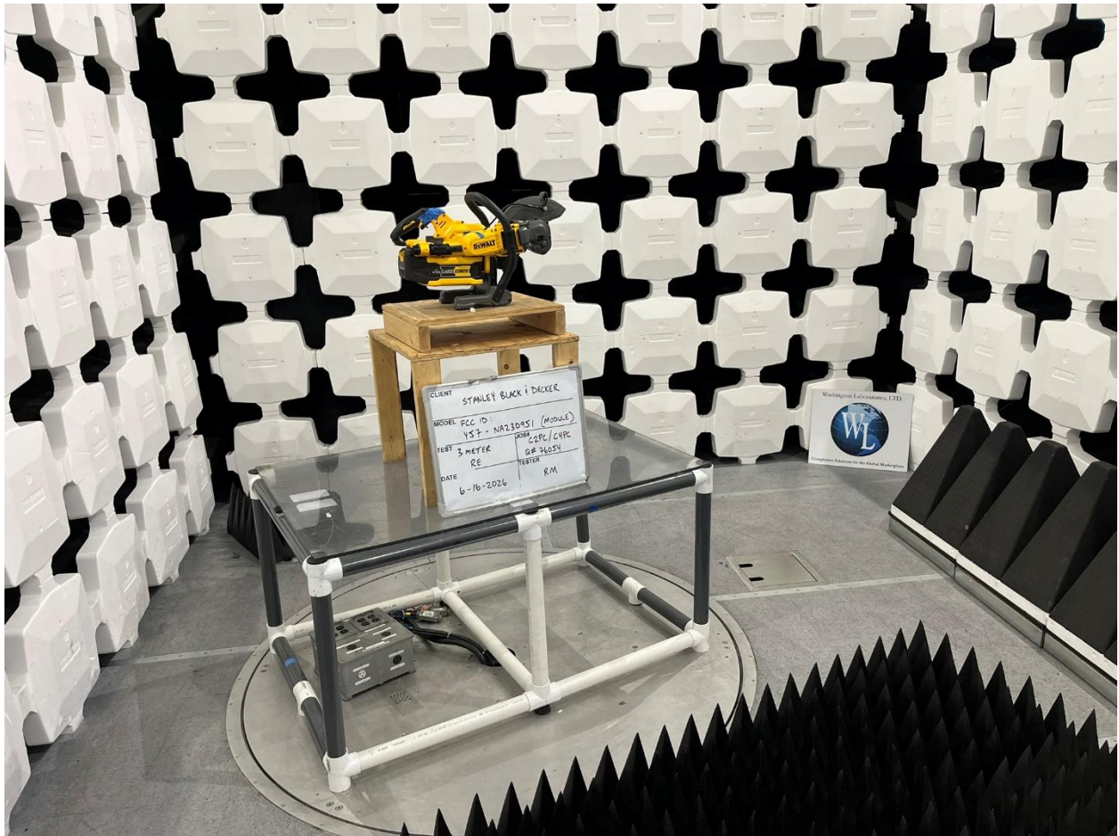
Above 1GHz Radiated Emissions, View 4
