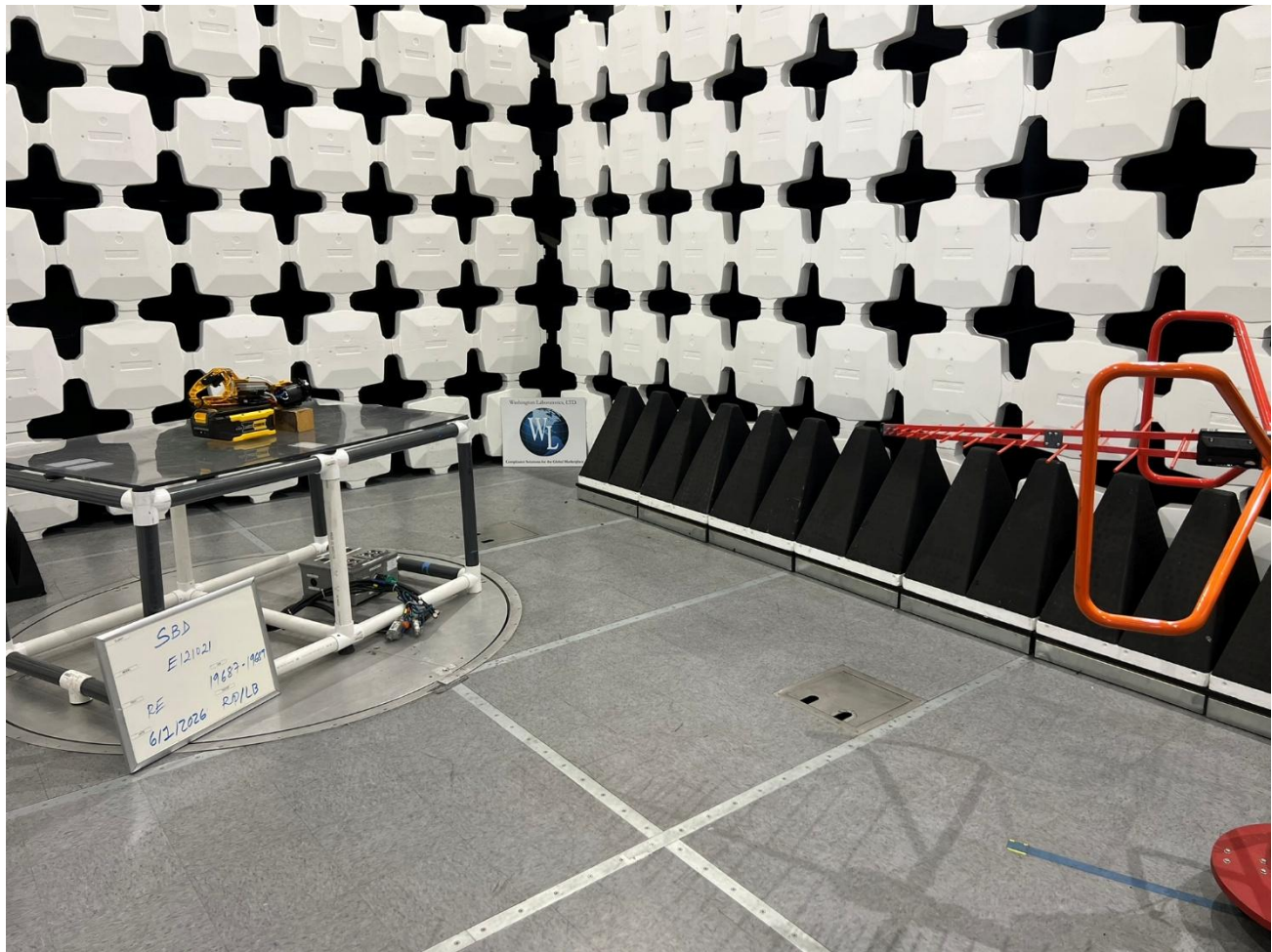
30MHz to 1GHz Radiated Emissions, View 1
