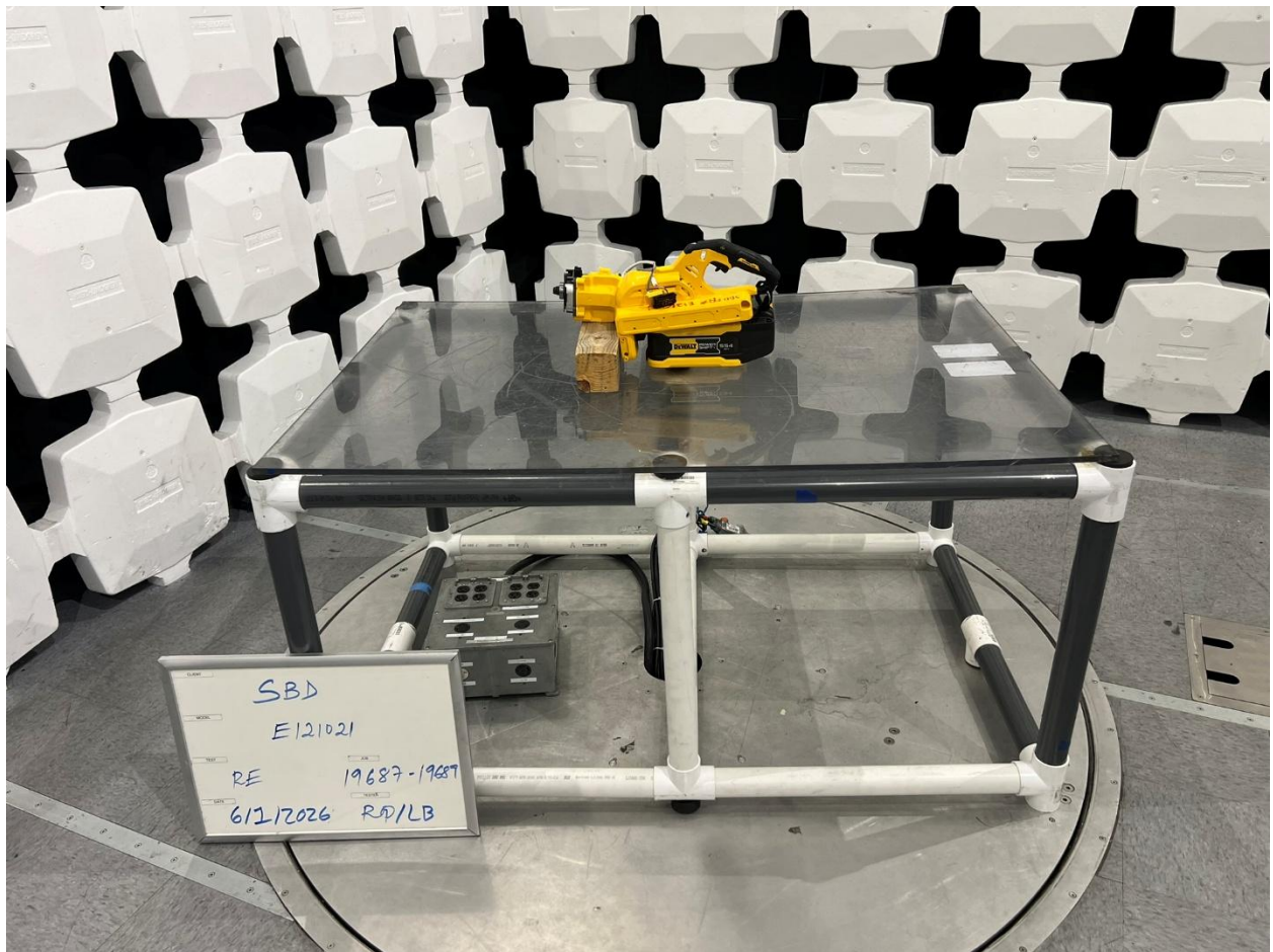
30MHz to 1GHz Radiated Emissions, View 2
