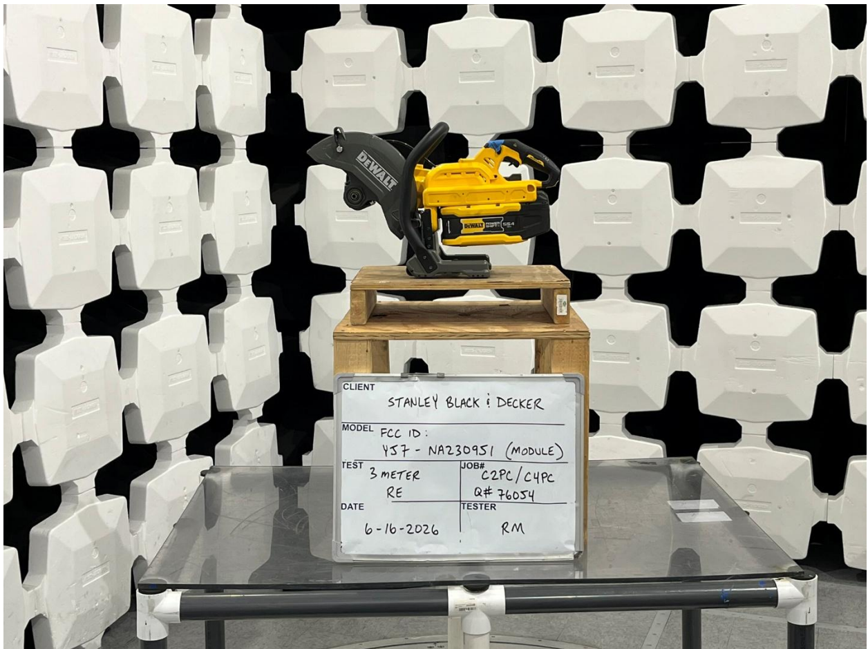
Above 1GHz Radiated Emissions, View 3
