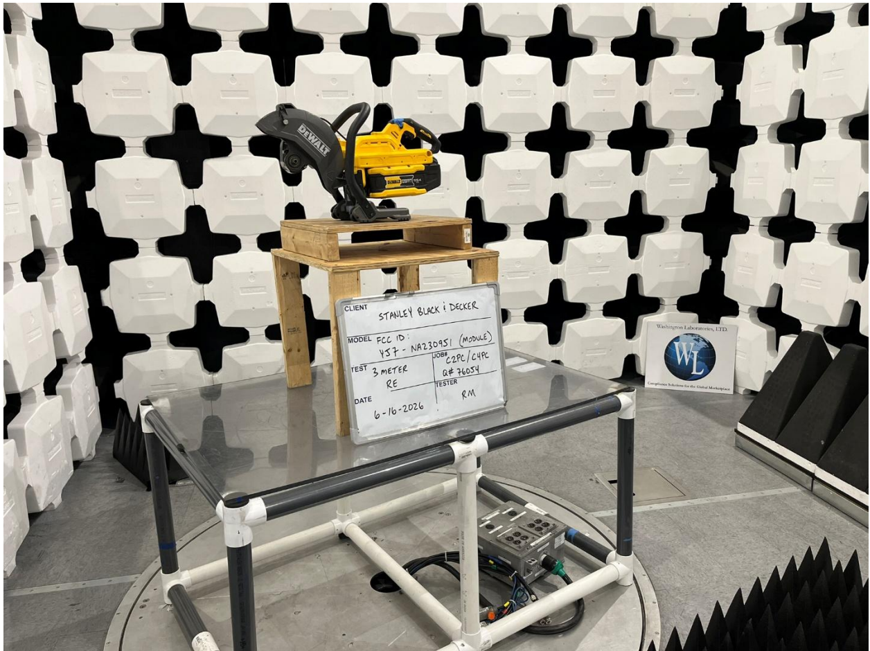
Above 1GHz Radiated Emissions, View 2
