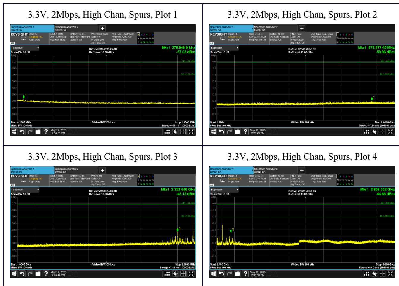
Figure 23: High Channel, 2Mbps ( \pi/4 DQPSK) Conducted Spurious, 3.3V, 250kHz to 5GHz
