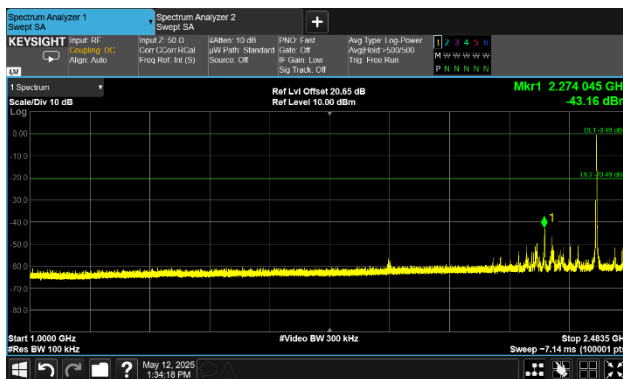
3.3V, 2Mbps, Low Chan, Spurs, Plot 3
