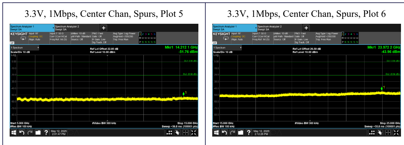
Figure 16: Center Channel, 1Mbps (GFSK) Conducted Spurious, 3.3V, 5GHz to 25GHz
