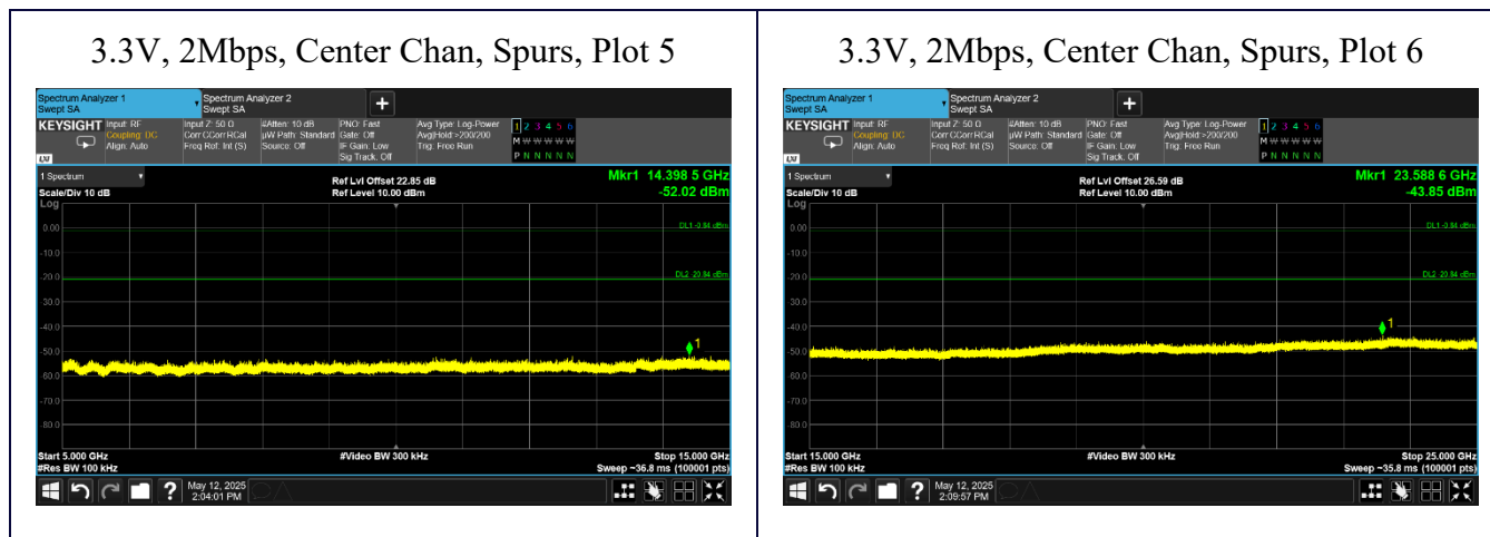
Figure 22: Center Channel, 2Mbps ( \pi/4 DQPSK) Conducted Spurious, 3.3V, 5GHz to 25GHz
