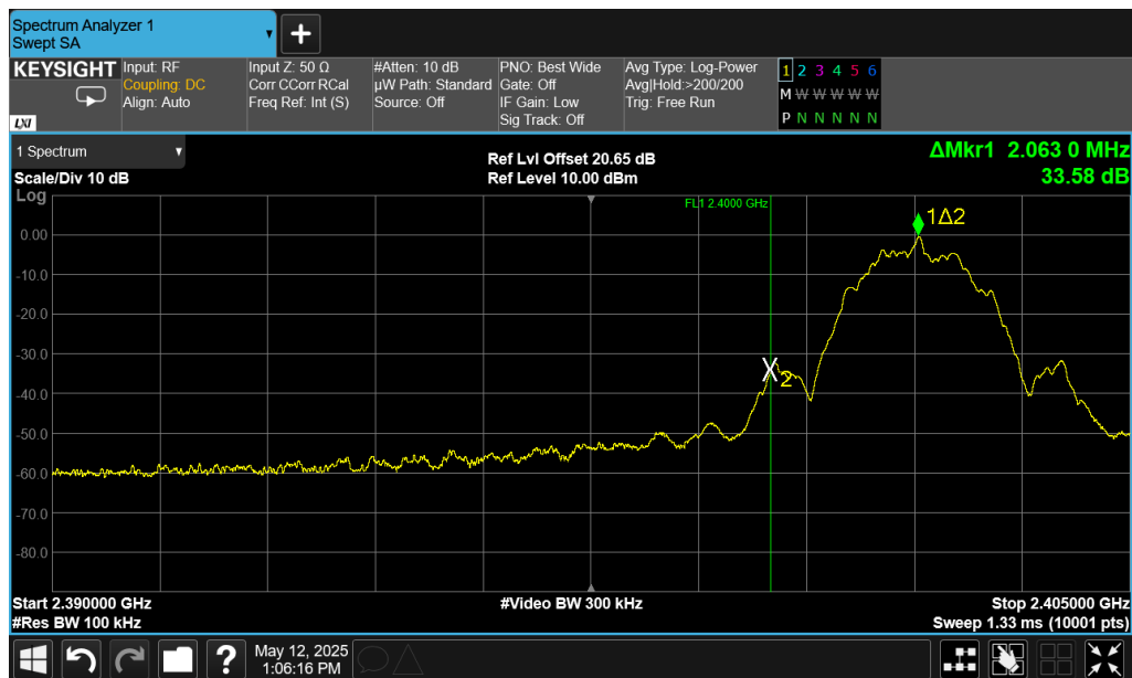
Figure 11: Low Channel Band-Edge, 2Mbps (2DH5), 3.3V
