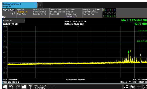
3.3V, 1Mbps, Low Chan, Spurs, Plot 3
