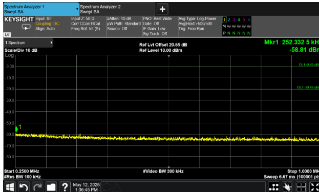
3.3V, 2Mbps, Low Chan, Spurs, Plot 1
