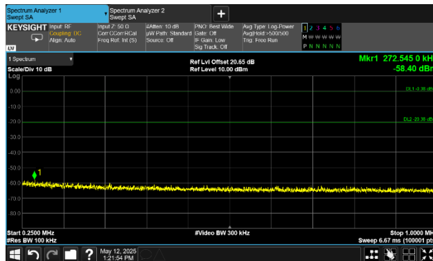
3.3V, 1Mbps, Low Chan, Spurs, Plot 1
