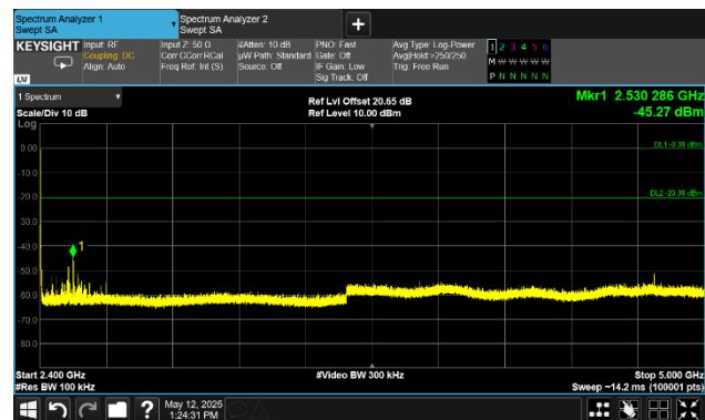
3.3V, 1Mbps, Low Chan, Spurs, Plot 4
