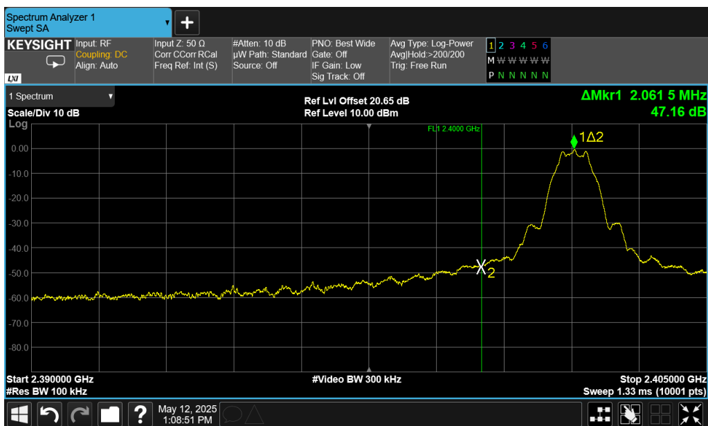
Figure 9: Low Channel Band-Edge, 1Mbps (DH5), 3.3V
