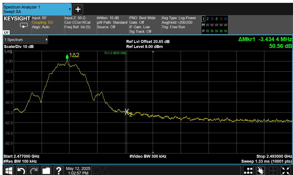
Figure 12: High Channel Band-Edge, 2Mbps (2DH5), 3.3V
