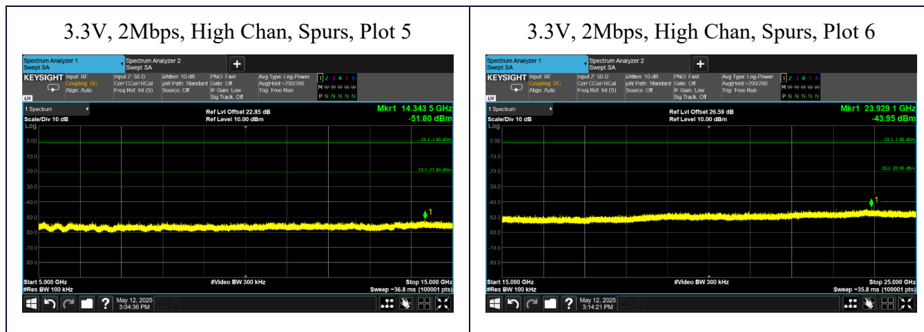
Figure 24: High Channel, 2Mbps ( \pi/4 DQPSK) Conducted Spurious, 3.3V, 5GHz to 25GHz
