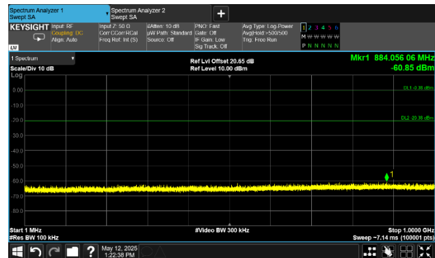
3.3V, 1Mbps, Low Chan, Spurs, Plot 2
