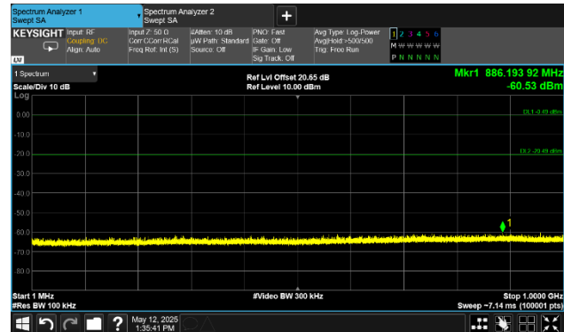
3.3V, 2Mbps, Low Chan, Spurs, Plot 2
