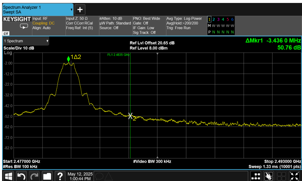
Figure 10: High Channel Band-Edge, 1Mbps (DH5), 3.3V
