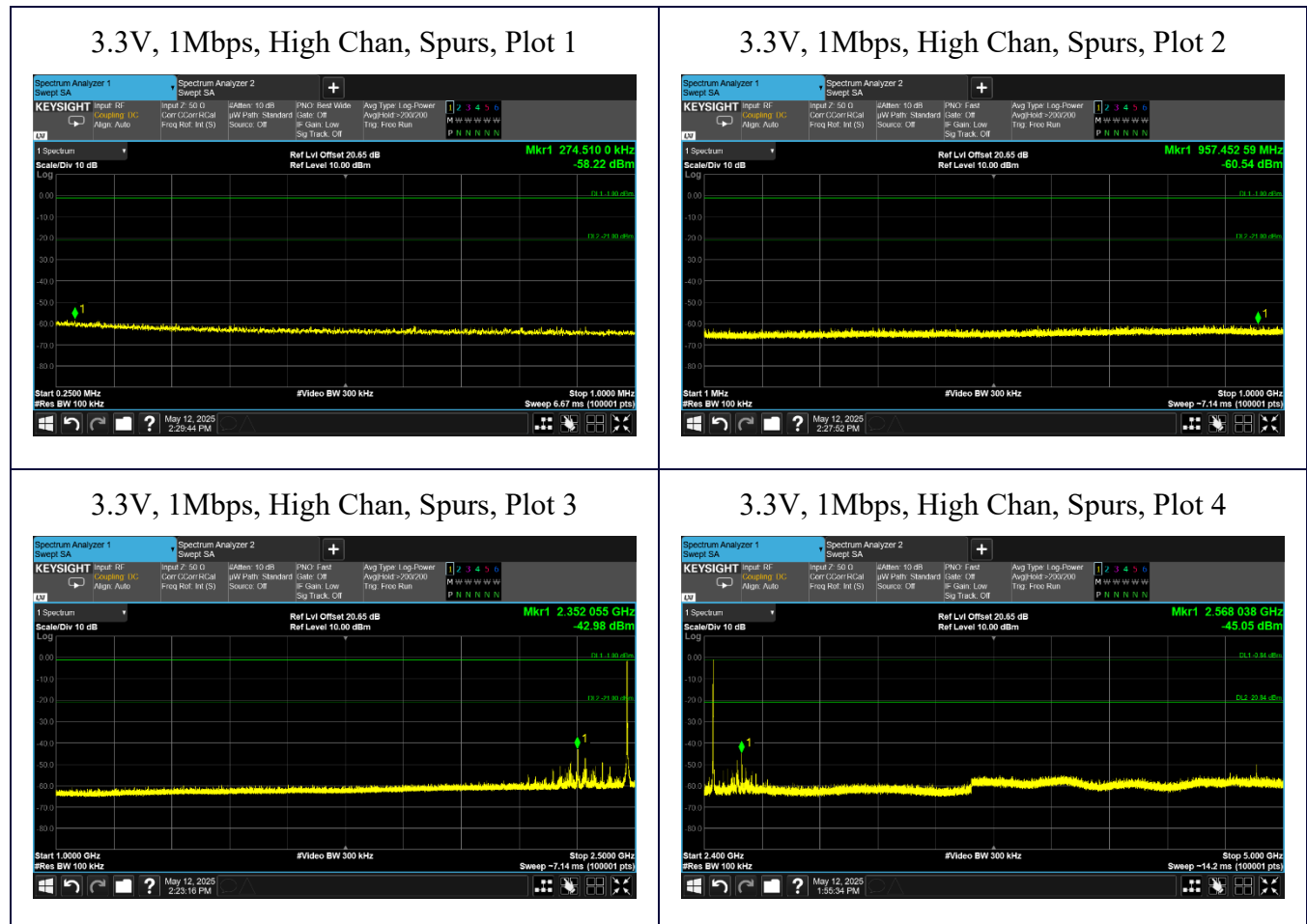
Figure 17: High Channel, 1Mbps (GFSK) Conducted Spurious, 3.3V, 250kHz to 5GHz
