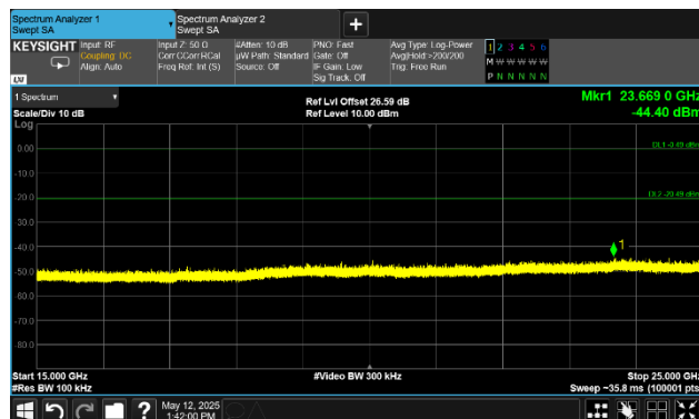
3.3V, 2Mbps, Low Chan, Spurs, Plot 6
