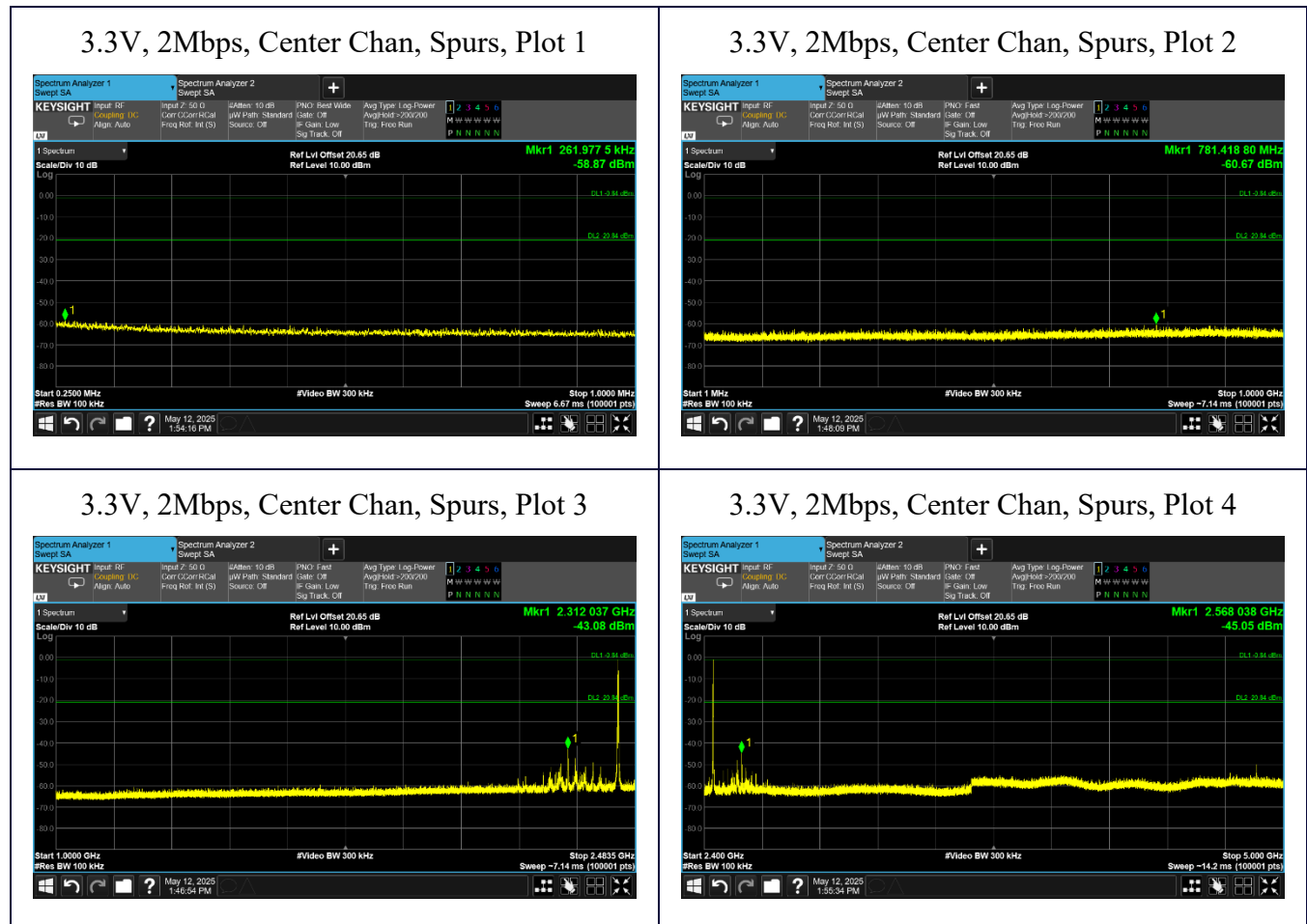
Figure 21: Center Channel, 2Mbps ( \pi/4 DQPSK) Conducted Spurious, 3.3V, 250kHz to 5GHz
