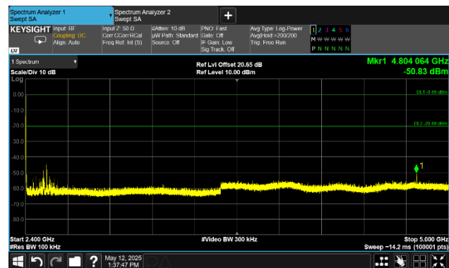
3.3V, 2Mbps, Low Chan, Spurs, Plot 4
