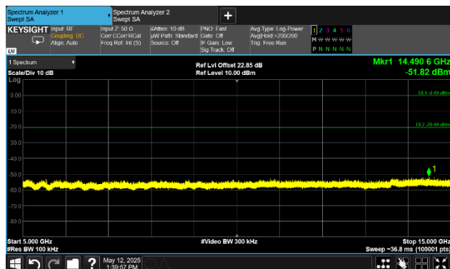
3.3V, 2Mbps, Low Chan, Spurs, Plot 5
