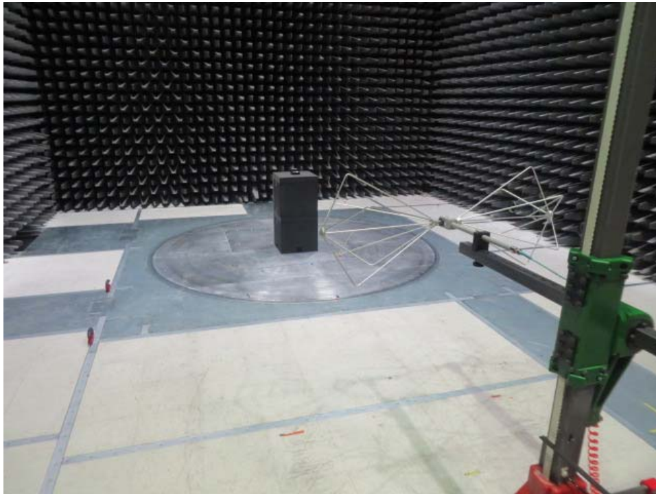
Radiated below 1 GHz
