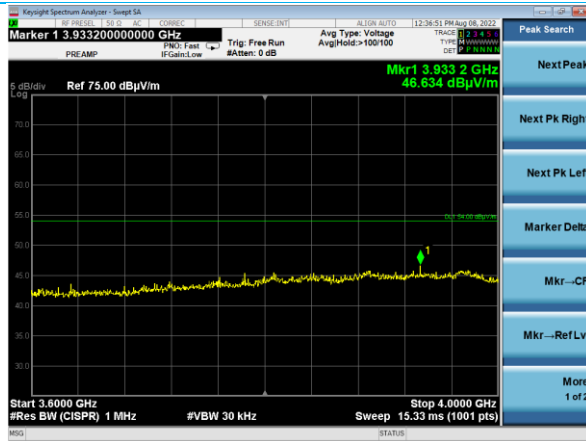
3600-4000 MHz Horizontal Polarity EUT Vertical Tx High
