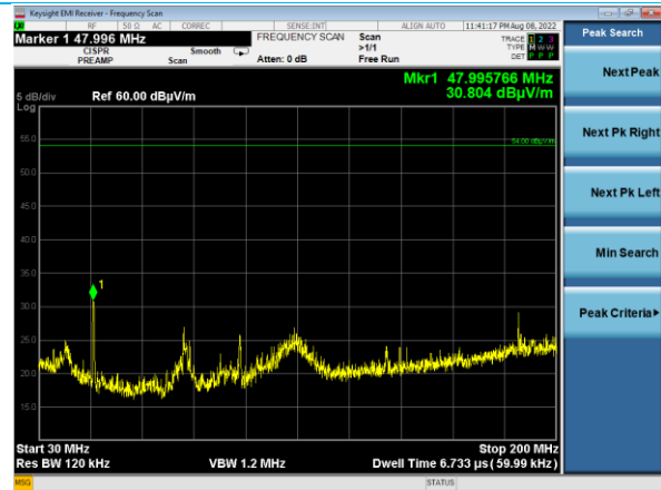
30-200 MHz Vertical Polarity EUT Vertical
