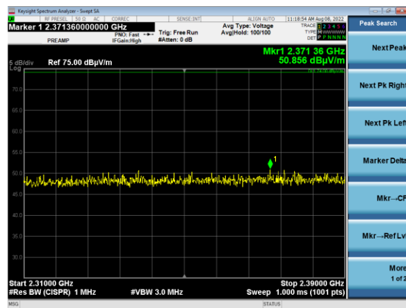
2310-2390 MHz Vertical Polarity EUT Vertical Tx Low Peak Measurement
