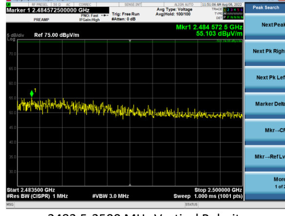
2483.5-2500 MHz Vertical Polarity EUT Vertical Tx High Peak Measurement
