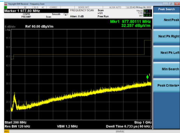
200-1000 MHz Vertical Polarity EUT Vertical
