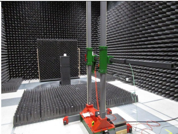
Above 1 GHz Radiated Emissions
