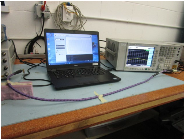
Conducted Measurements
