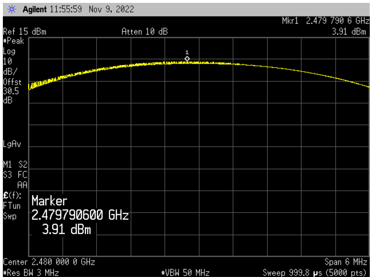
Figure 3: GFSK (1Mbps) – High Channel, Peak Power Output
