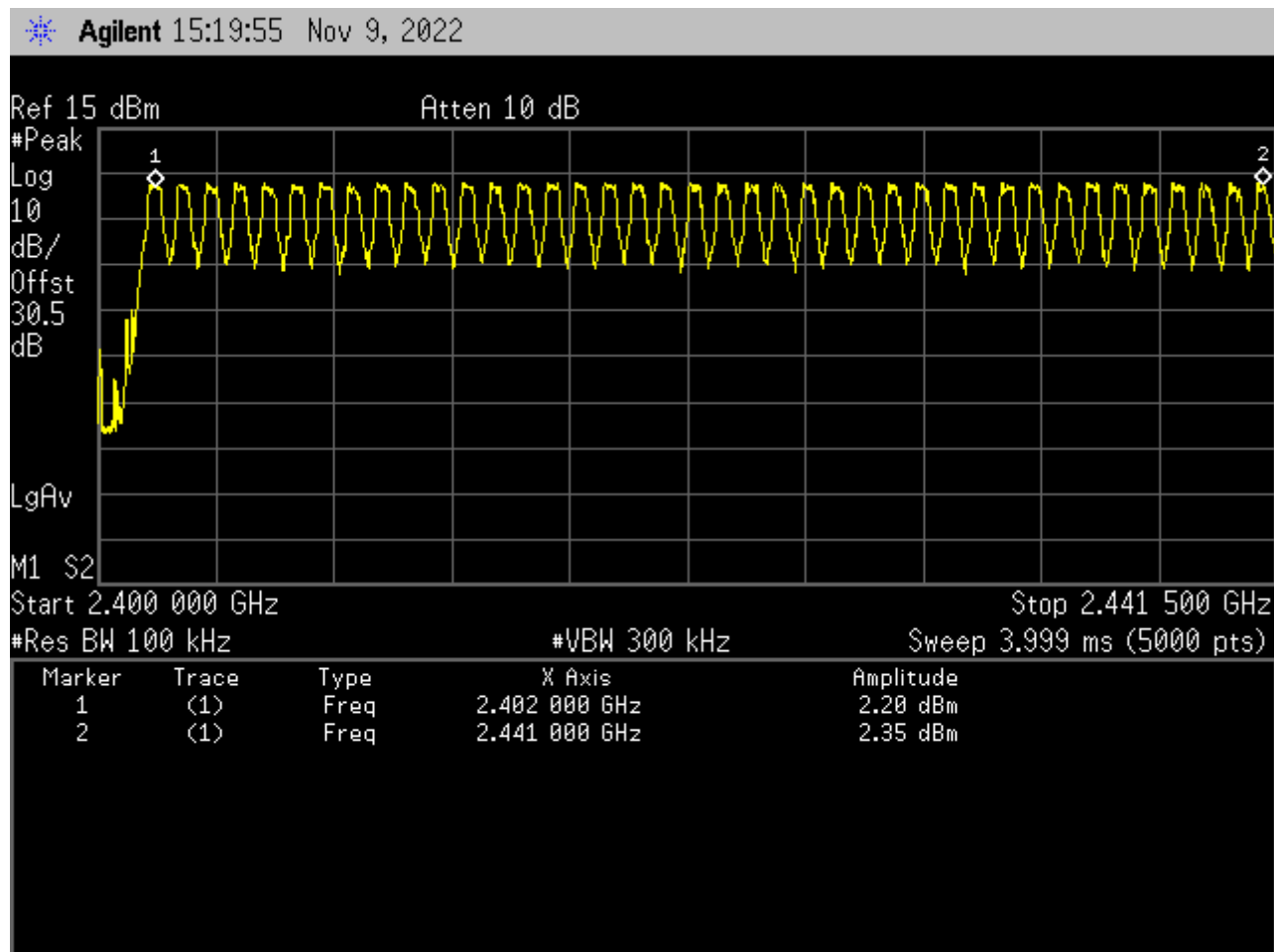
Figure 19: GFSK (1Mbps) – Number of Channels Used, Plot 1
