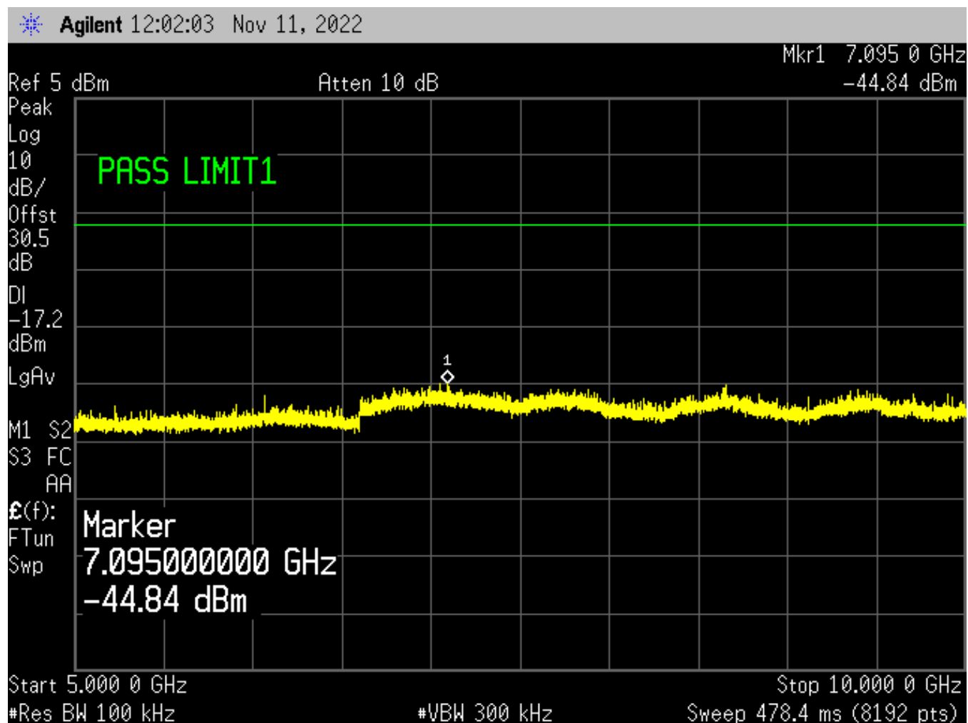
Figure 48: GFSK (1Mbps) Center Channel, Conducted Spurious – Plot 3
