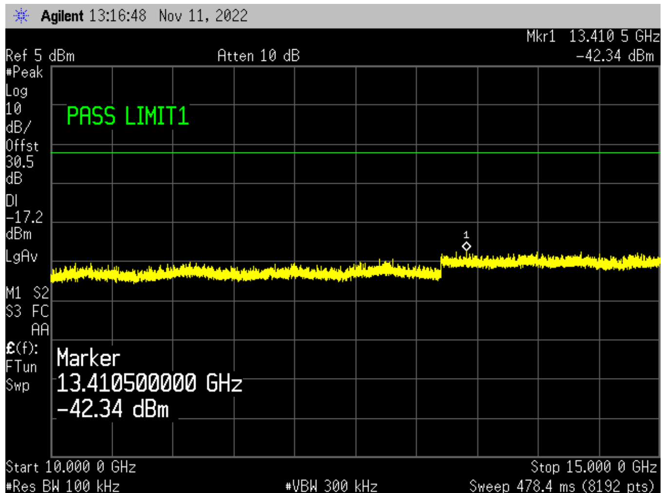
Figure 43: GFSK (1Mbps) Low Channel, Conducted Spurious – Plot 4
