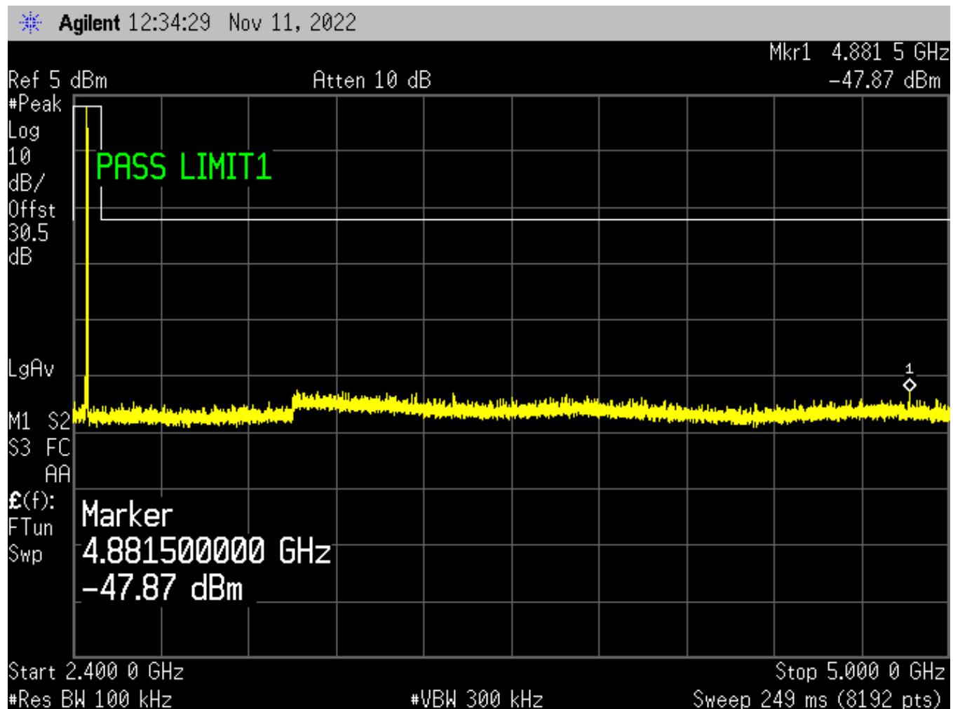
Figure 65: 8DPSK (3Mbps) Center Channel, Conducted Spurious – Plot 2
