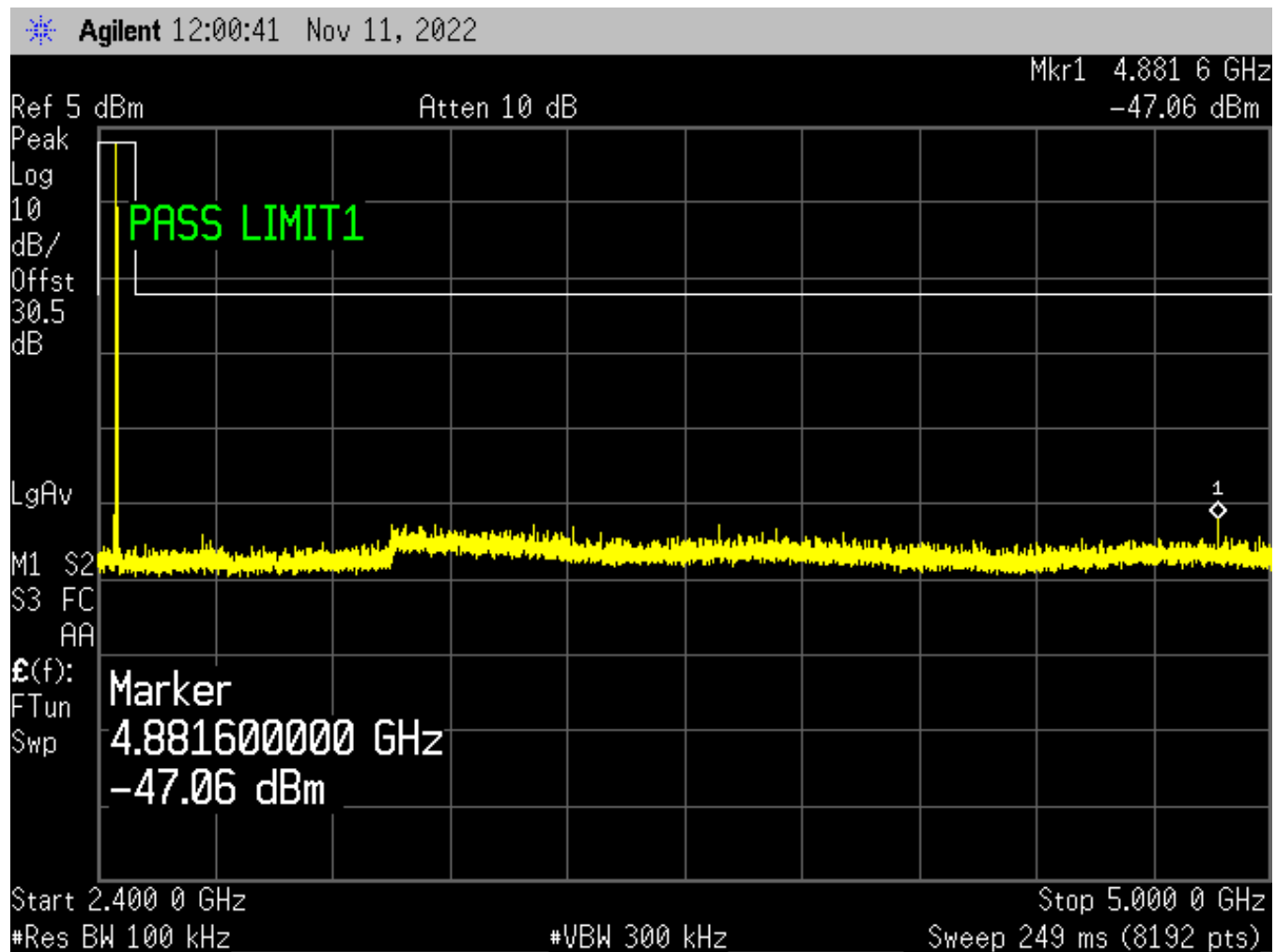
Figure 47: GFSK (1Mbps) Center Channel, Conducted Spurious – Plot 2
