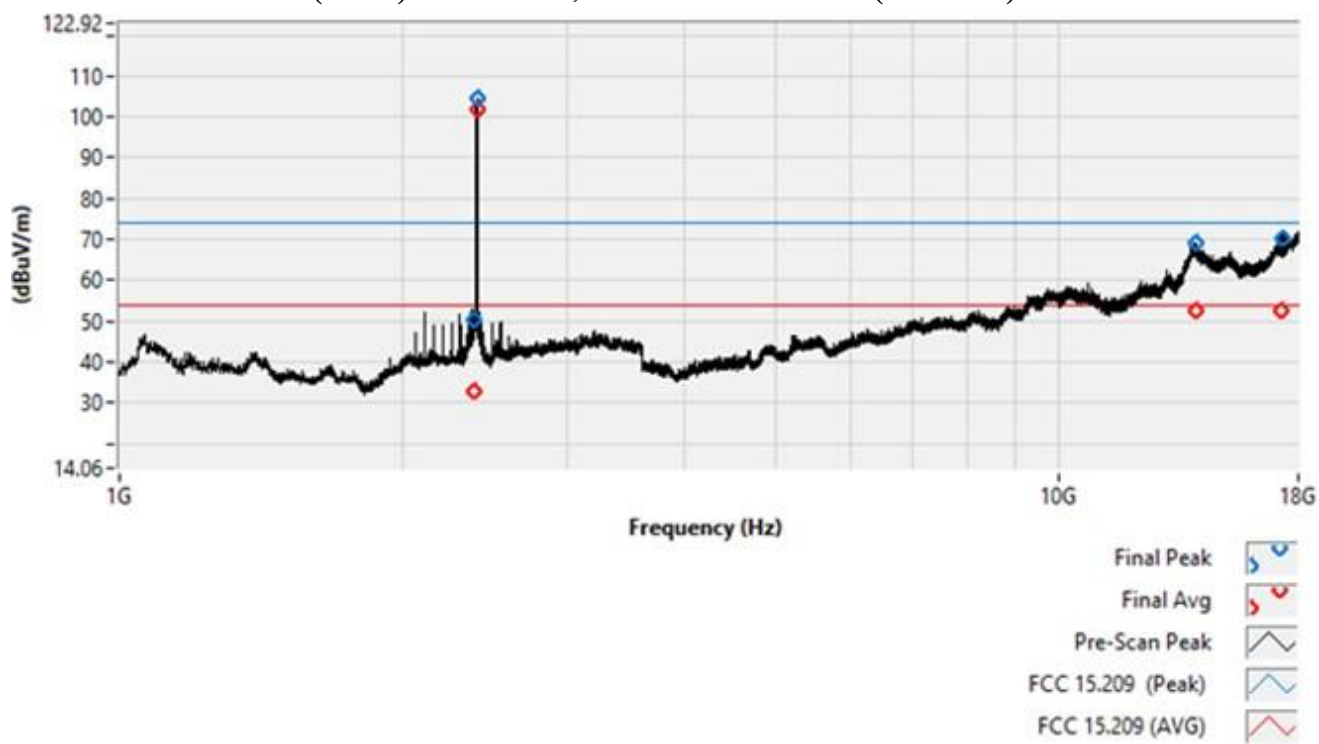
(GFSK) Low Channel, Pre-scan and Final Data (Horizontal)
