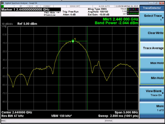
Mid Channel (2440 MHz)
