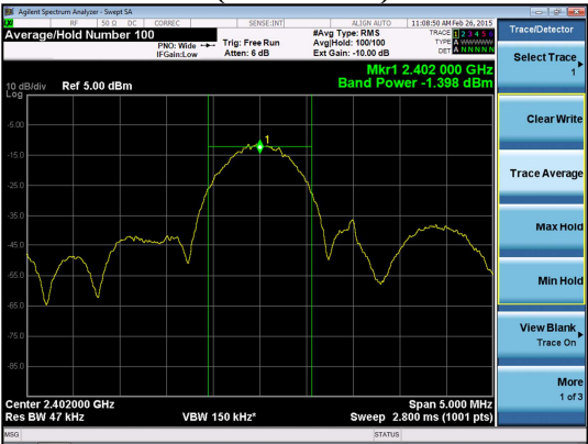
Plots Low Channel (2402 MHz)
