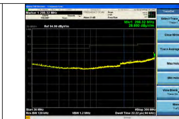
30-300 MHz Horizontal
