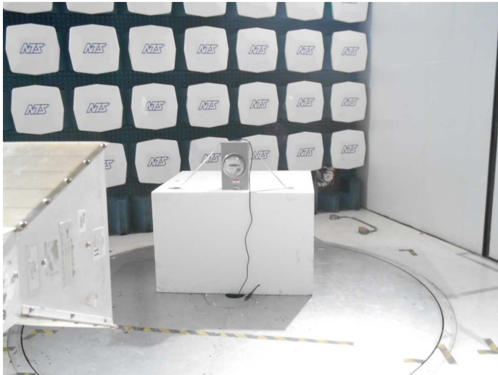
Radiated Emissions 1GHz-10GHz
