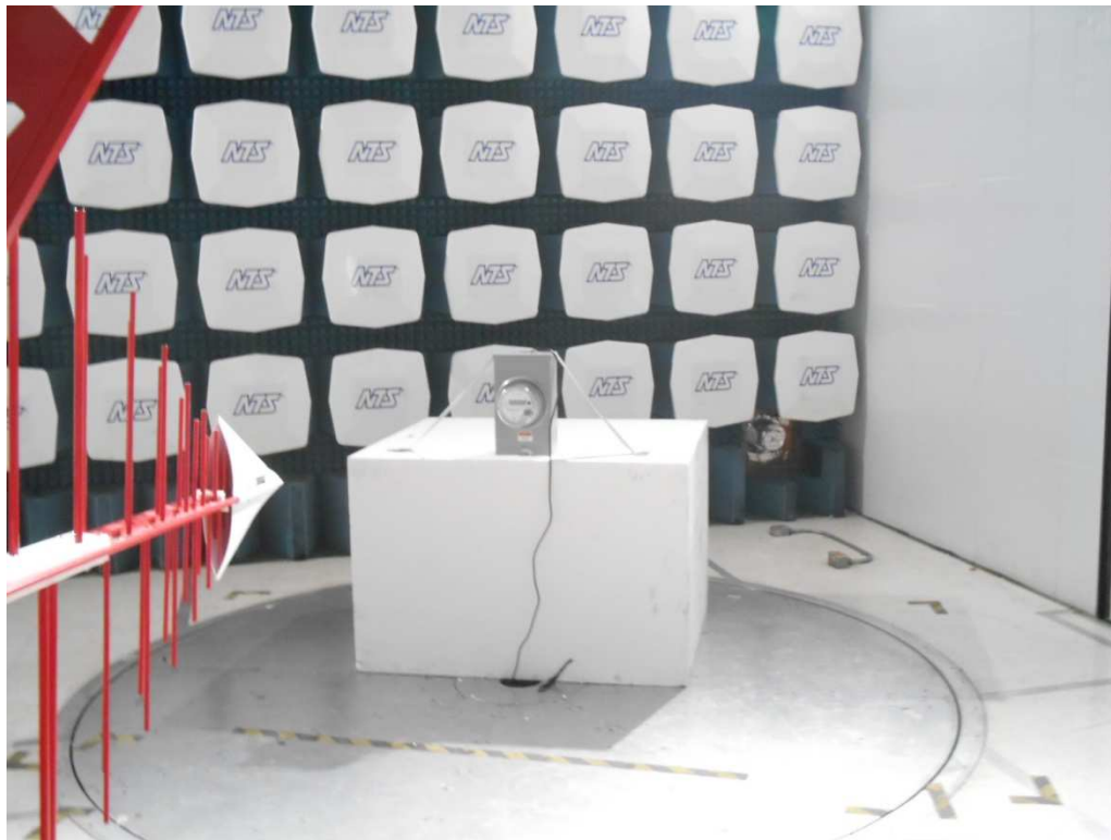
Radiated Emissions 30MHz-1GHz
