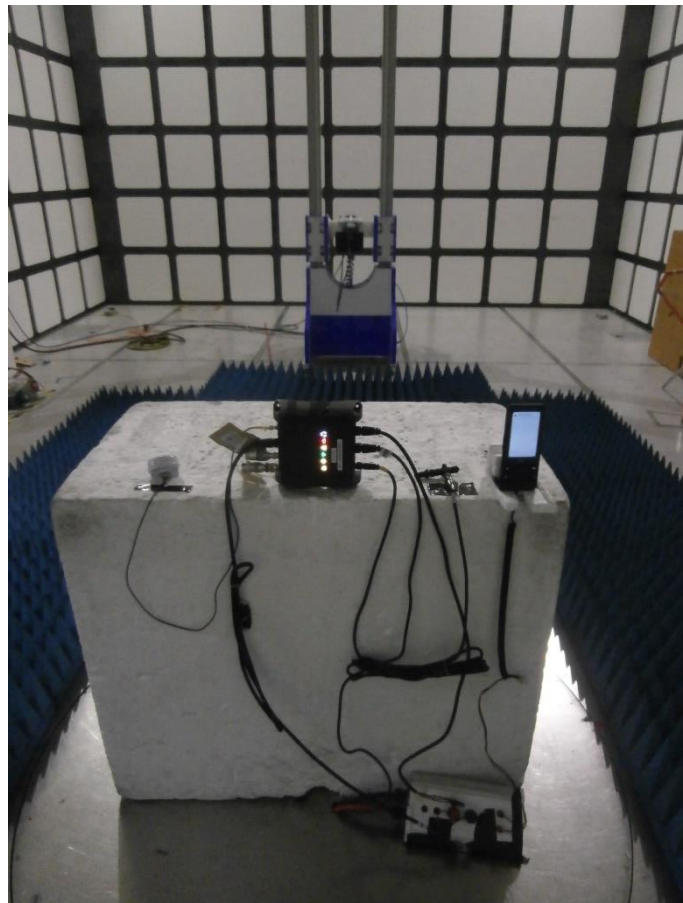
Figure 39 – Radiated Emissions, 1 GHz to 2 GHz, Orientation Y
