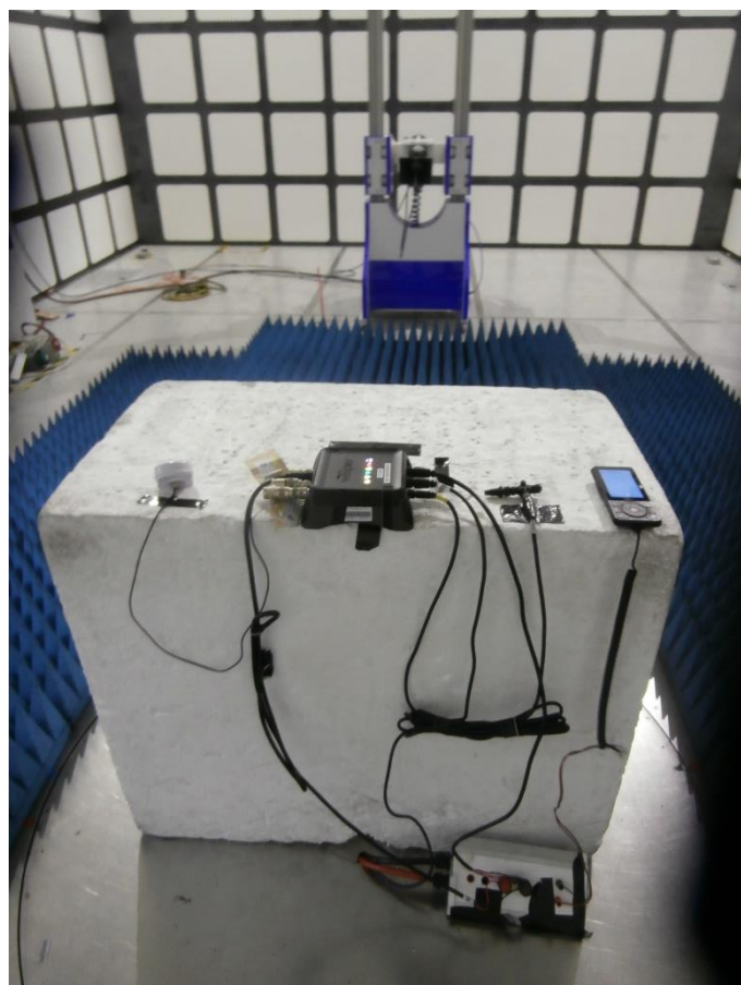
Figure 38 – Radiated Emissions, 1 GHz to 2 GHz, Orientation X
