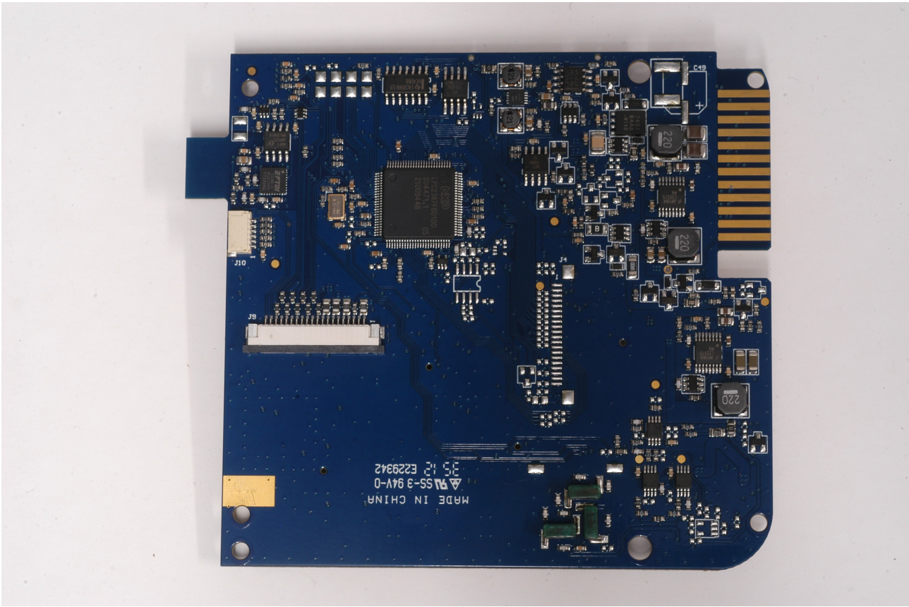
WMX850 AIS Engine – Bottom side
