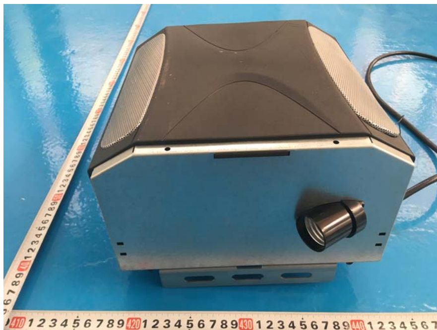
EUT (628FCACC) – Right View
