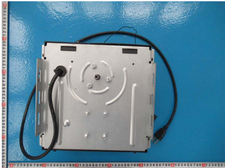
EUT (628CC) – BottomView
