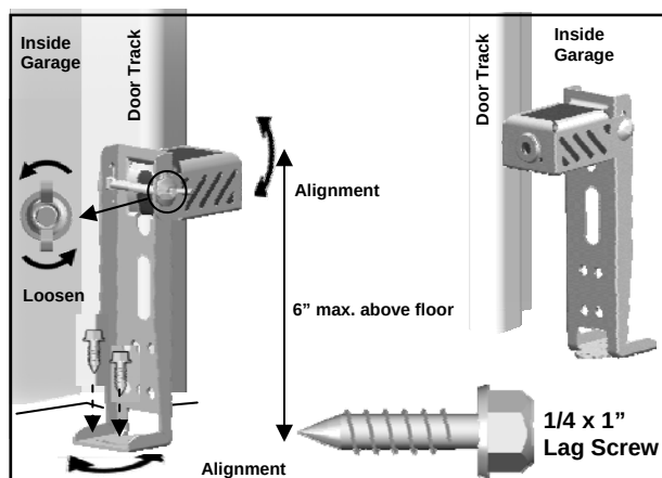
Fig. 2 (Floor Mount)
