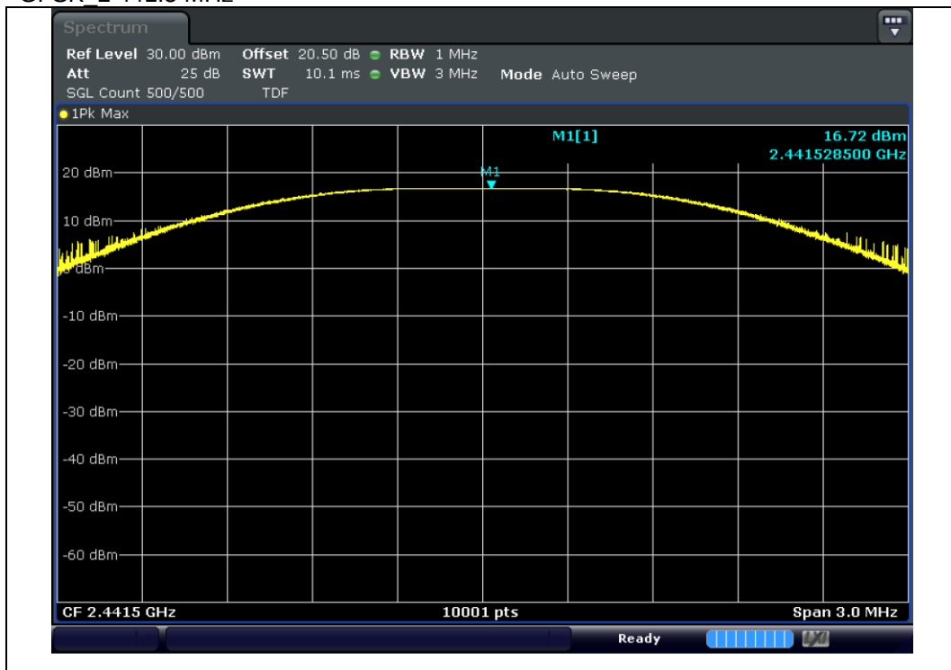
GFSK 2 441.5 MHz
