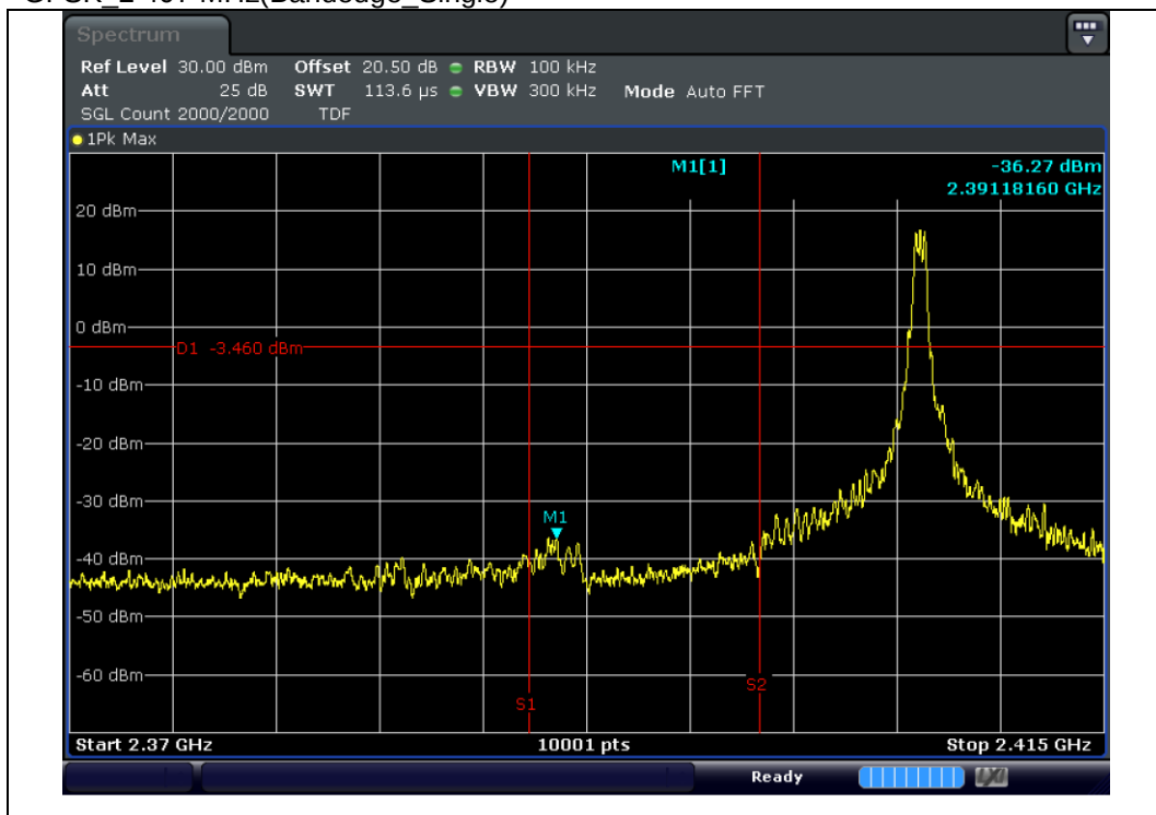
GFSK_2 407 MHz(Bandedge_Single)
