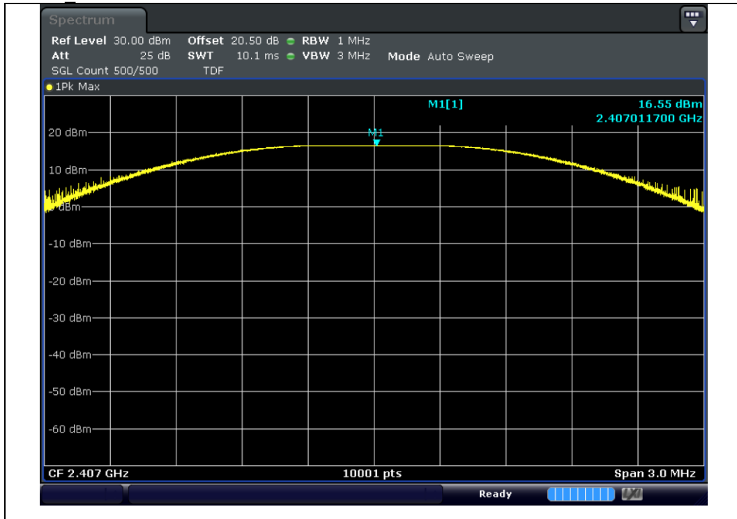
GFSK 2 407 MHz
