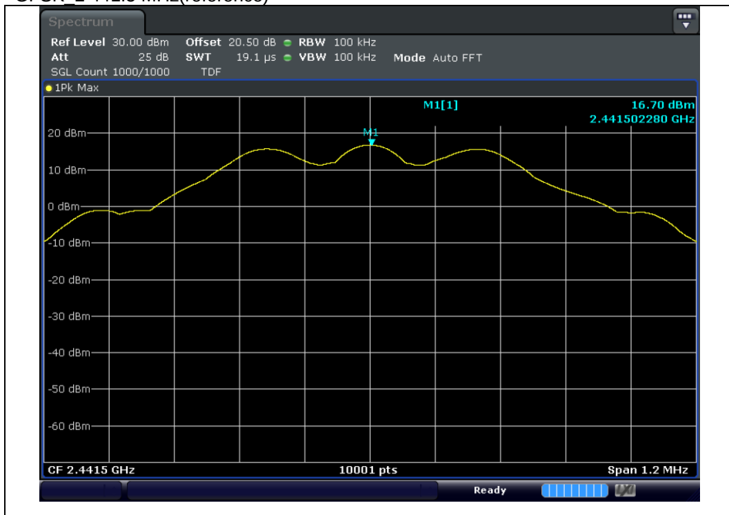
GFSK 2 441.5 MHz(reference)
