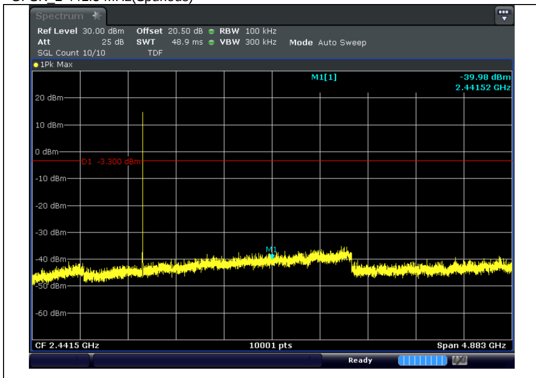
GFSK_2 441.5 MHz(Spurious)
