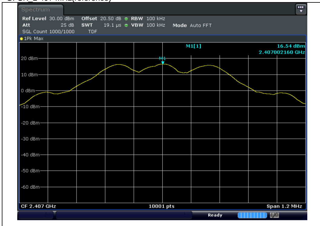
GFSK 2 407 MHz(reference)
