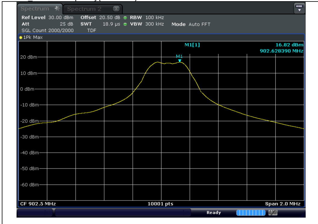
GFSK_Lowest Frequency(reference)
