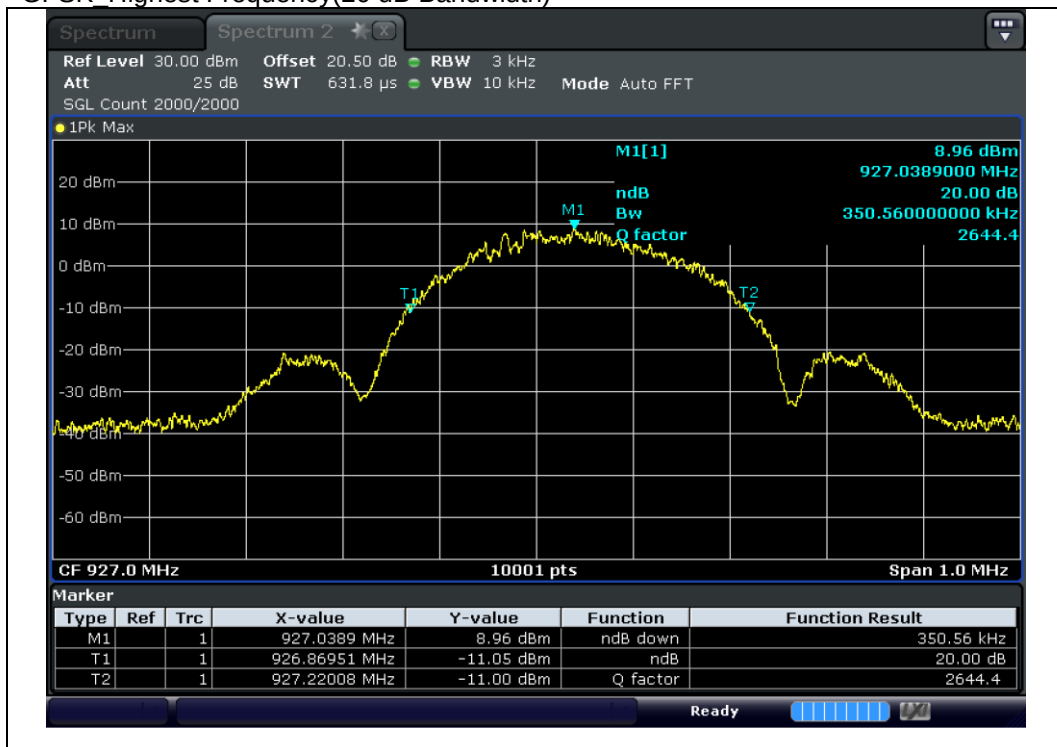
GFSK_Highest Frequency(20 dB Bandwidth)
