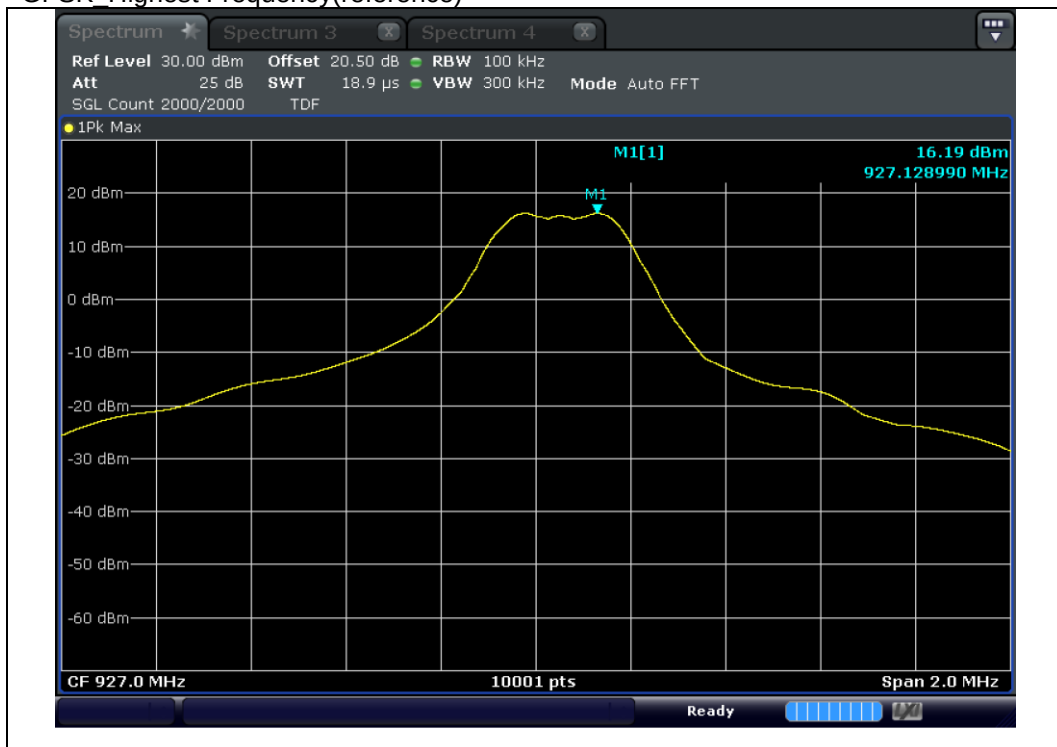
GFSK_Highest Frequency(reference)
