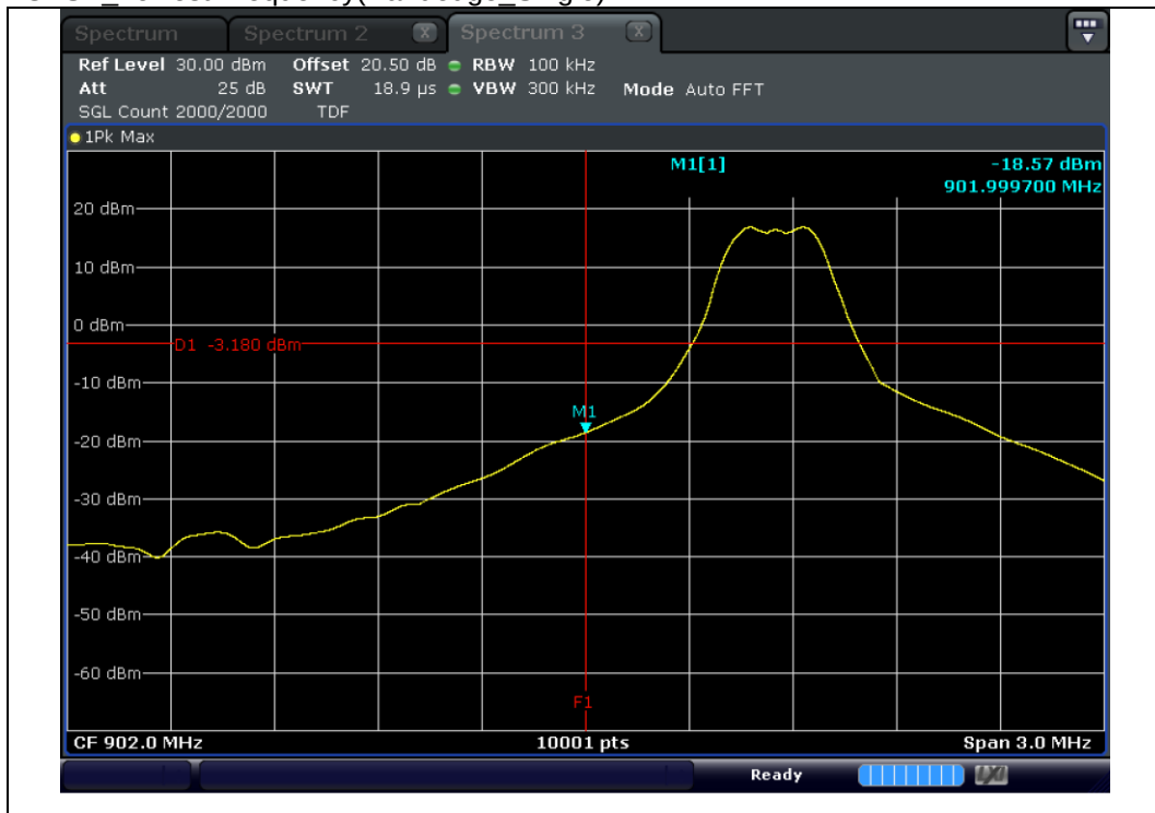
GFSK_Lowest Frequency(Bandedge_Single)
