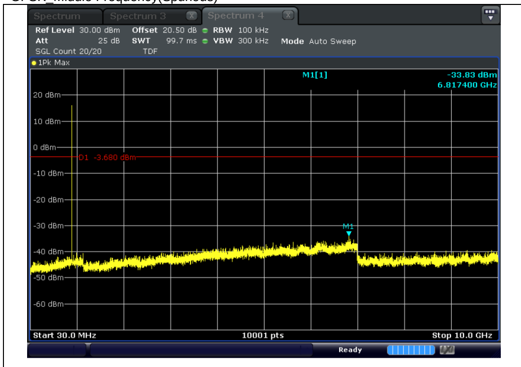
GFSK Middle Frequency(Spurious)
