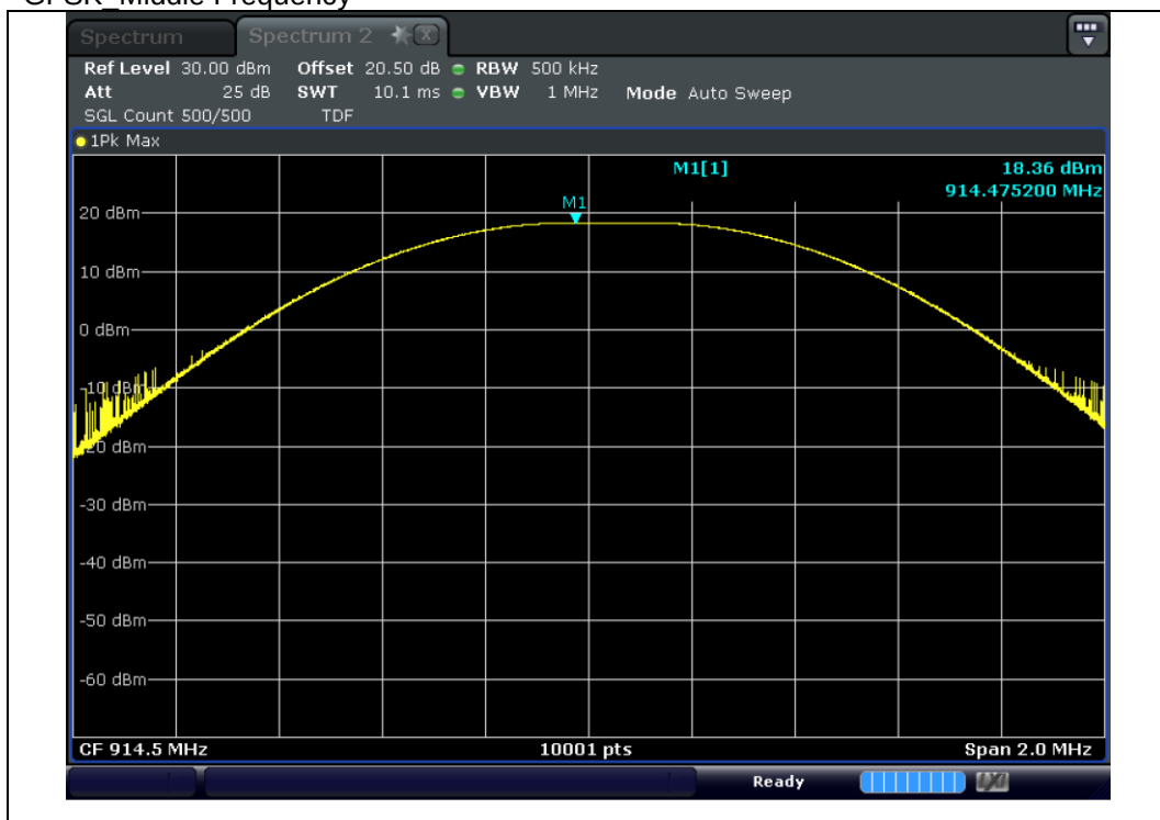
GFSK Middle Frequency
