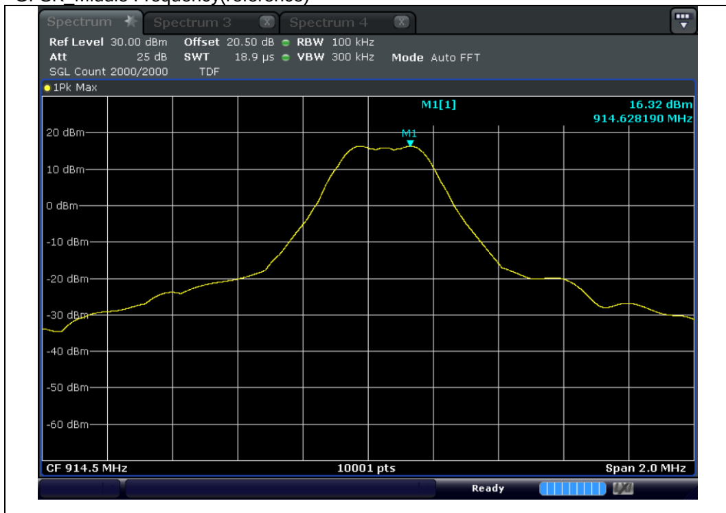
GFSK Middle Frequency(reference)
