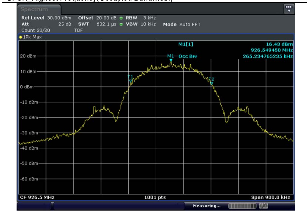
GFSK_Highest Frequency(Occupied Bandwidth)
