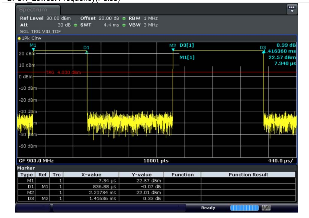
GFSK_Lowest Frequency(Pulse)
