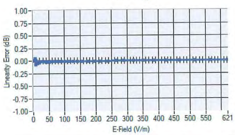
Linearity
