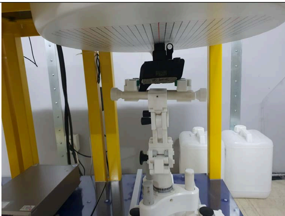
Bottom of Device 0 mm from Phantom Top view
