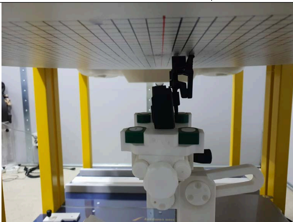
Bottom of Device 0 mm from Phantom Side view
