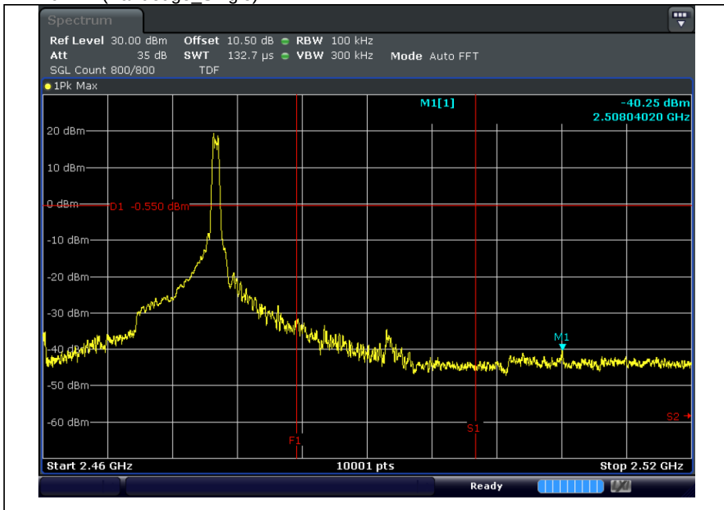
2 476 MHz(Bandedge_Single)
