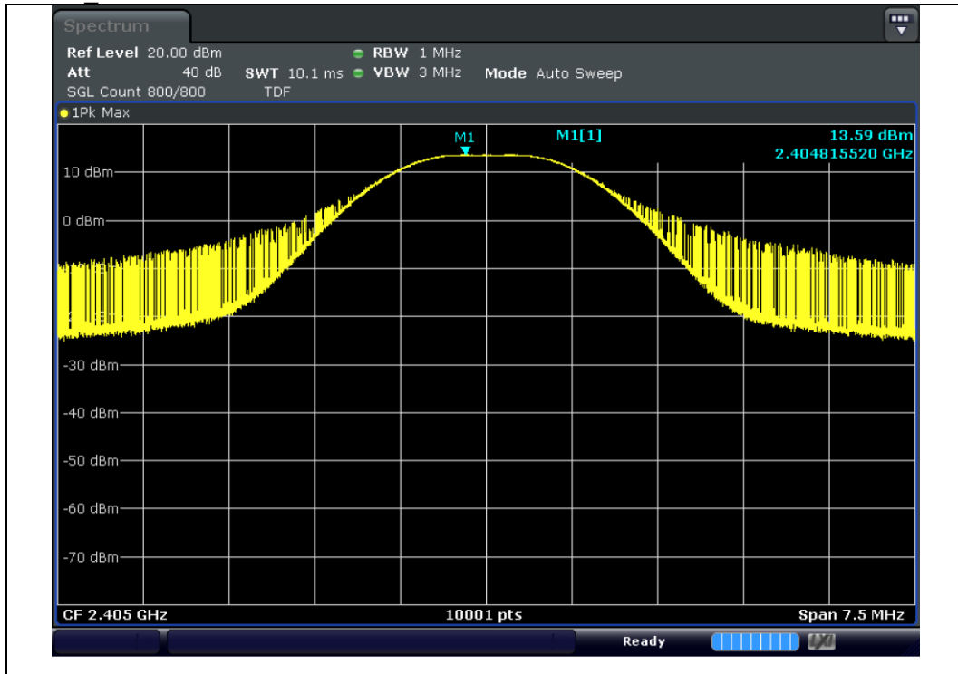
GFSK 2 405 MHz
