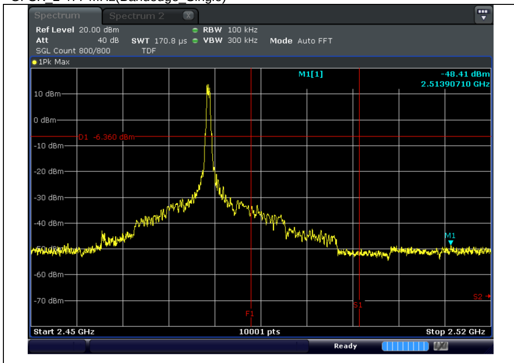
GFSK_2 477 MHz(Bandedge_Single)
