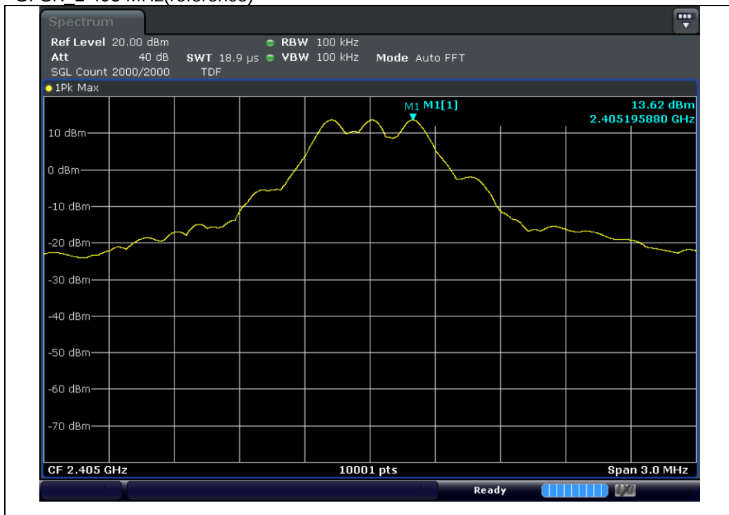
GFSK 2 405 MHz(reference)
