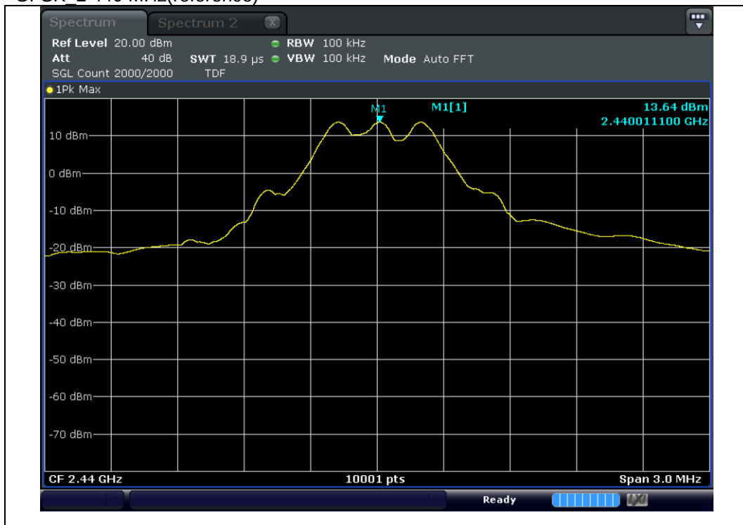
GFSK 2 440 MHz(reference)
