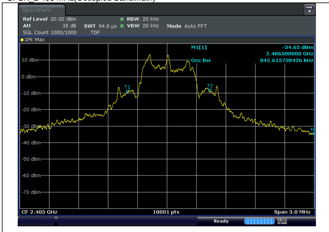
GFSK_2 405 MHz(Occupied Bandwidth)
