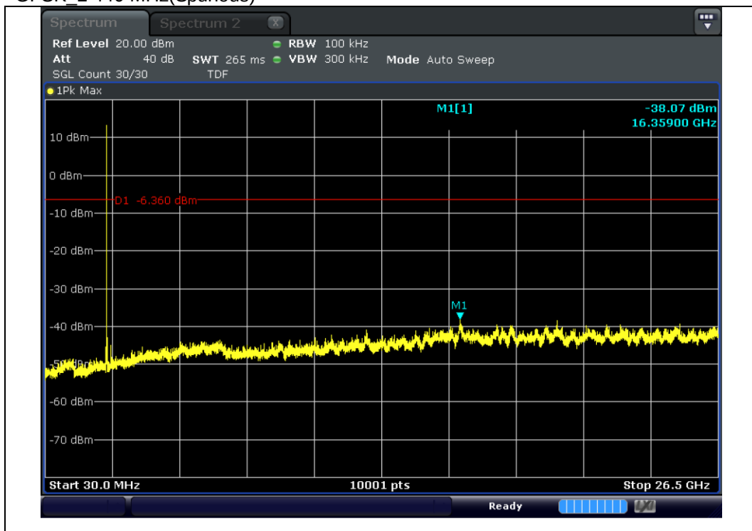
GFSK 2 440 MHz(Spurious)
