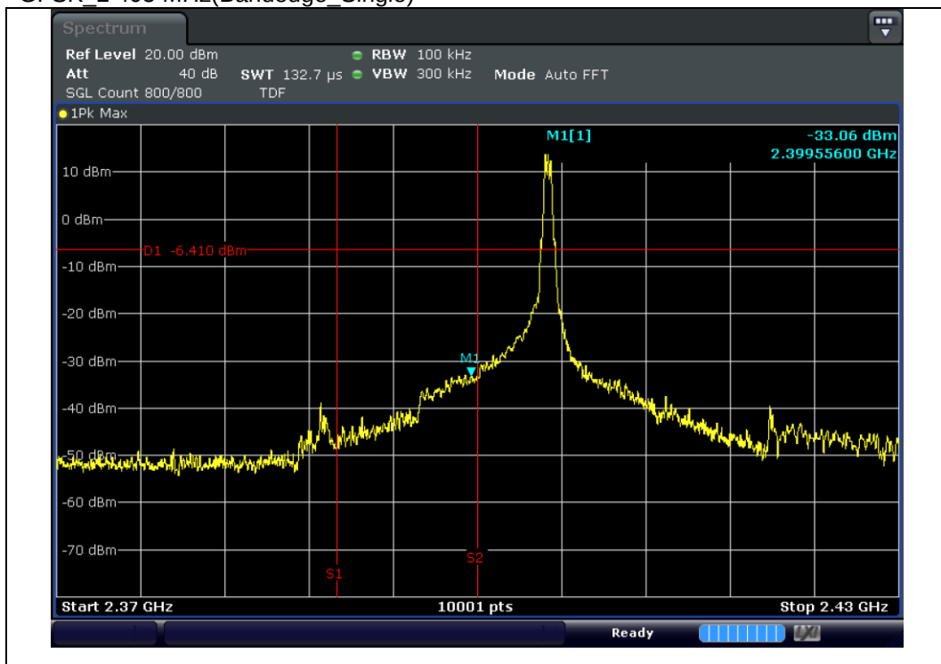
GFSK_2 405 MHz(Bandedge_Single)
