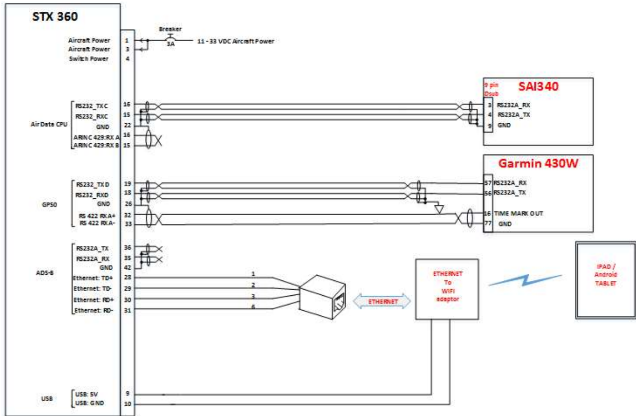
Figure 19: Installation of STX 360 with WAAS position source, encoder and optional output to table through WIFI
