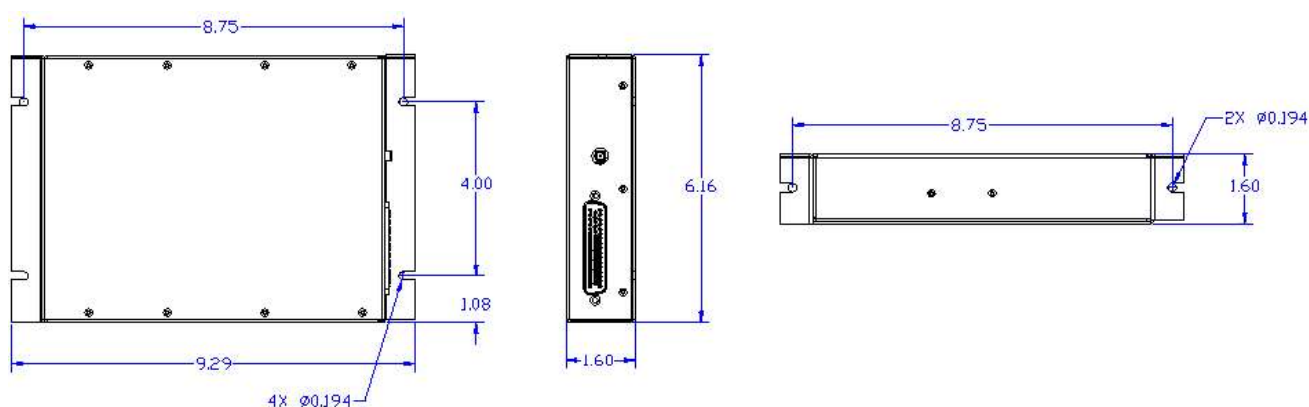
Figure 2: Physical dimensions of STX 360R remote
