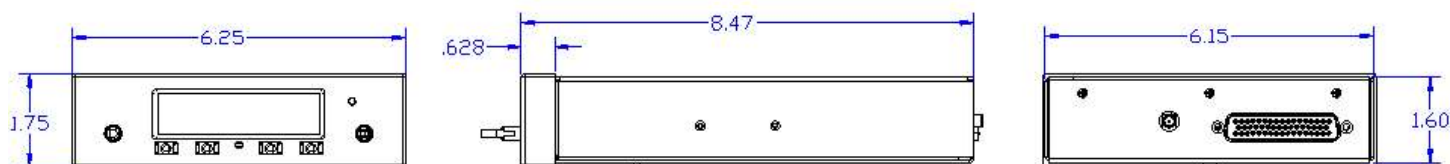
Figure 1: Physical dimensions of STX 360 panel mount
