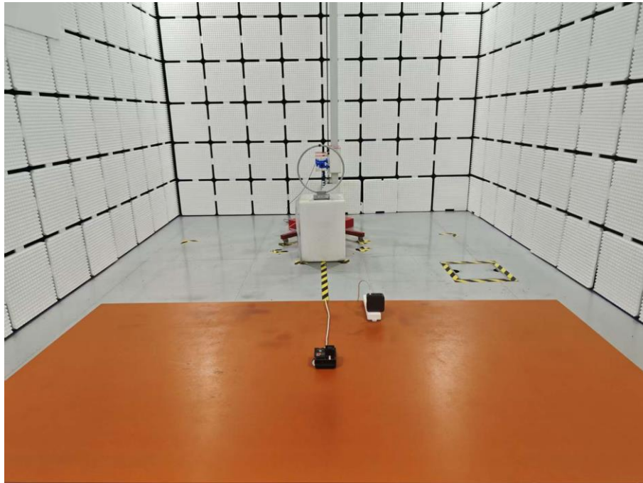
Radiated Emission Below 30MHz
