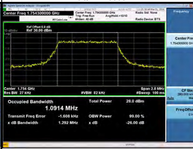
16QAM-20393
