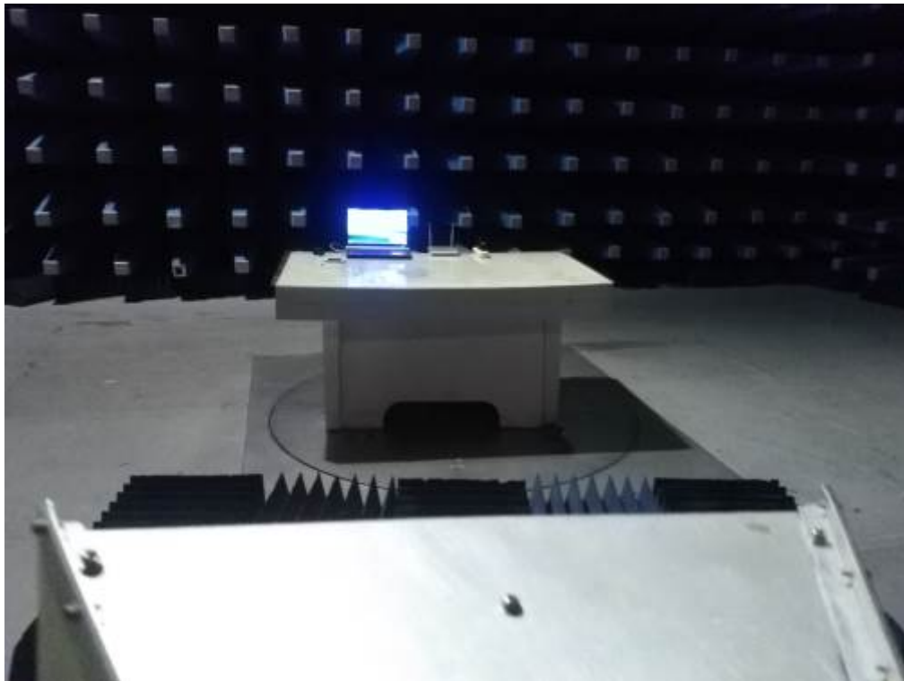
Radiated Emissions Test Setup Above 1GHz—Adapter: RD1200500-C55-8MG
