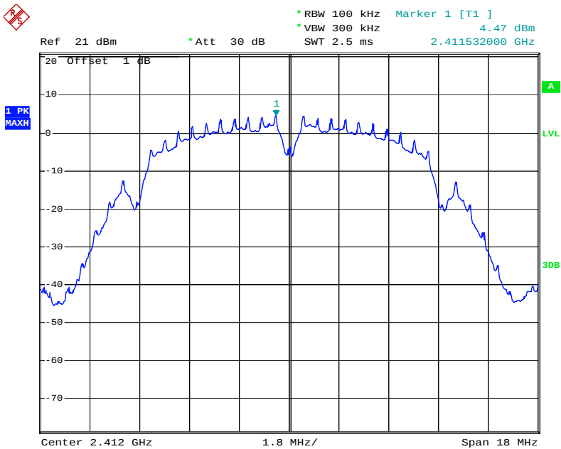
Power Spectral Density, 802.11b Low Channel (ANT 1#)
