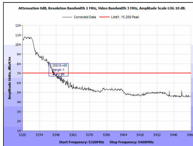
Radiated Band Edge, 802.11n 20 MHz, 5320 MHz, Both Chains, Peak
