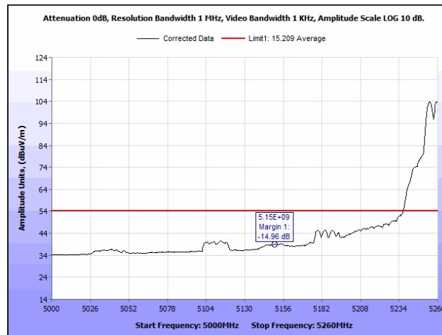
Radiated Band Edge, 802.11a 20 MHz, 5260 MHz, Both Chains, Average
