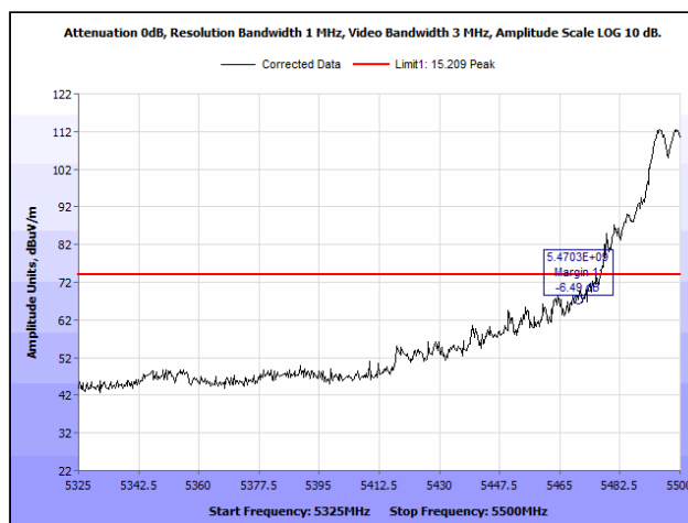
Radiated Band Edge, 802.11a 20 MHz, 5500 MHz, Both Chains, Peak
