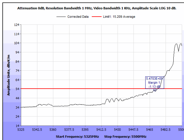
Radiated Band Edge, 802.11a 20 MHz, 5500 MHz, Both Chains, Average
