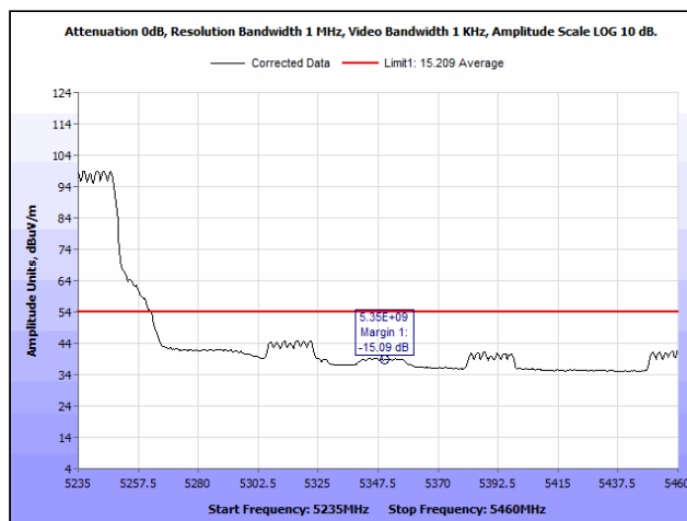
Radiated Band Edge, 802.11n 20 MHz, 5240 MHz, Both Chains, Average
