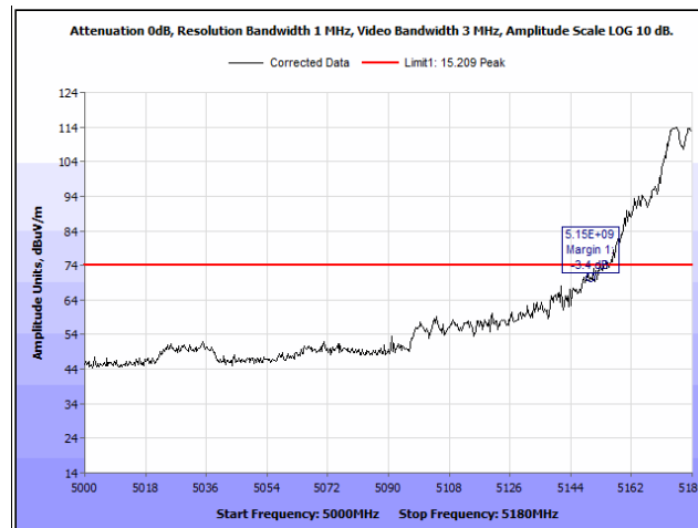
Radiated Band Edge, 802.11a 20 MHz, 5180 MHz, Both Chains, Peak
