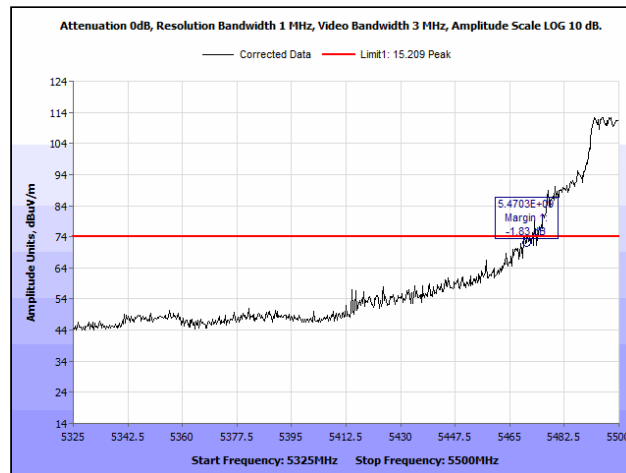
Radiated Band Edge, 802.11n 20 MHz, 5500 MHz, Both Chains, Peak
