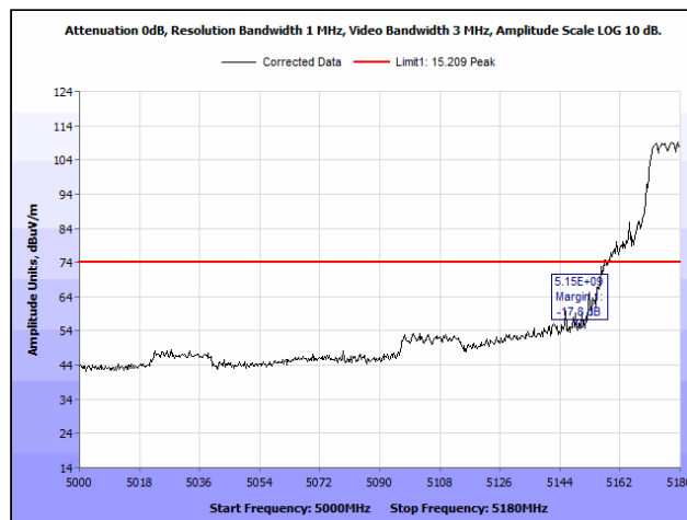
Radiated Band Edge, 802.11n 20 MHz, 5180 MHz, Both Chains, Peak
