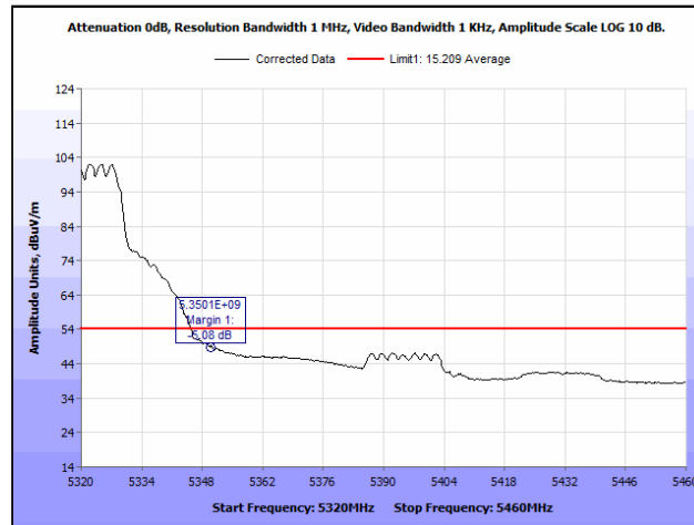
Radiated Band Edge, 802.11n 20 MHz, 5320 MHz, Both Chains, Average
