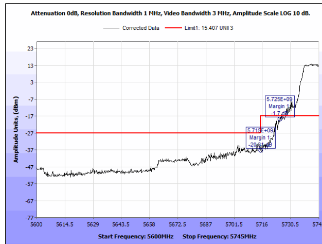
Radiated Band Edge, 802.11a 20 MHz, 5745 MHz, Both Chains
