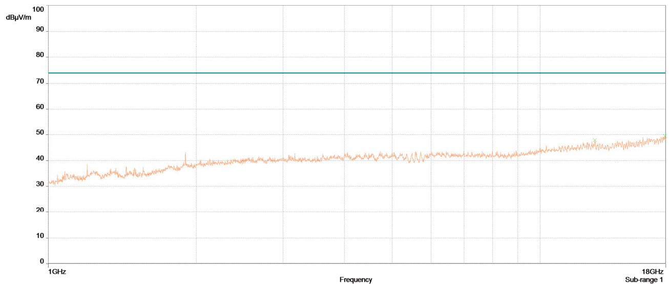
Radiated Spurious Emissions, 1GHz -18 GHz, BT Mid Channel, Peak (Worst Case Pol)
