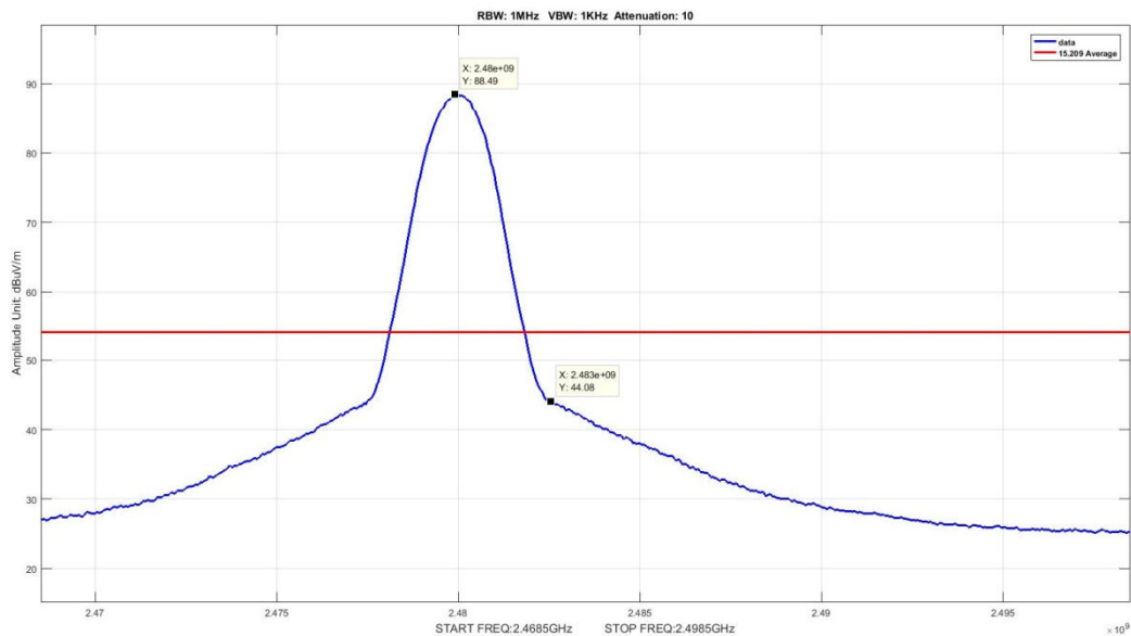
Radiated Emissions, BT BLE, Radiated Band Edge, High Average
