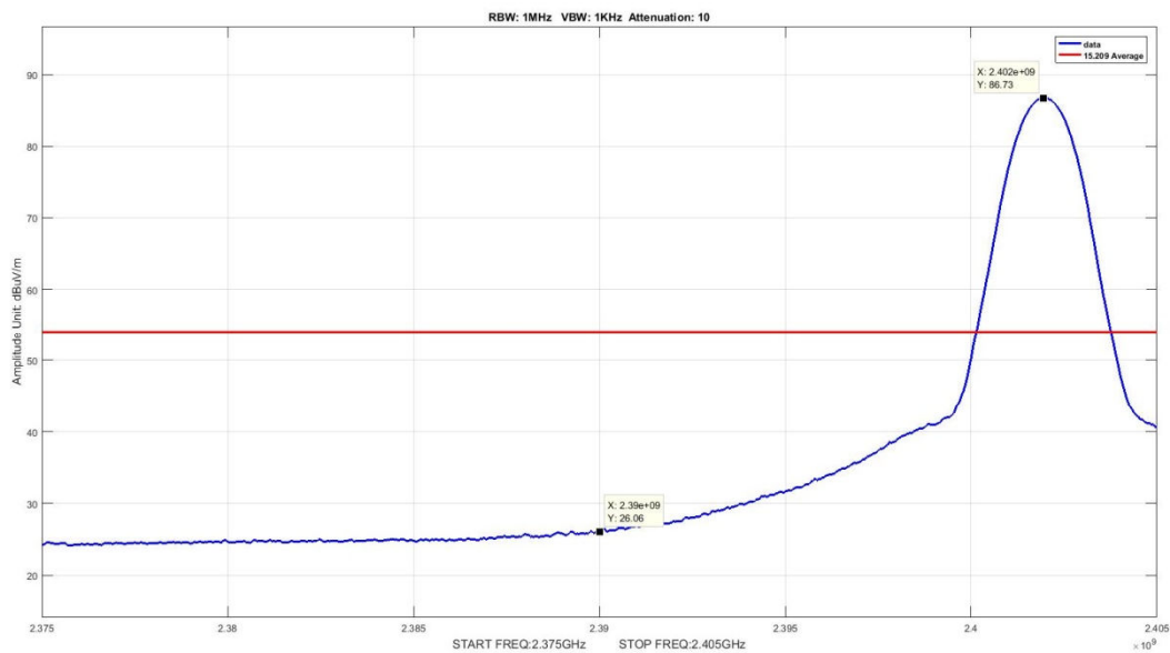
Radiated Emissions, BT BLE, Radiated Band Edge, Low Average
