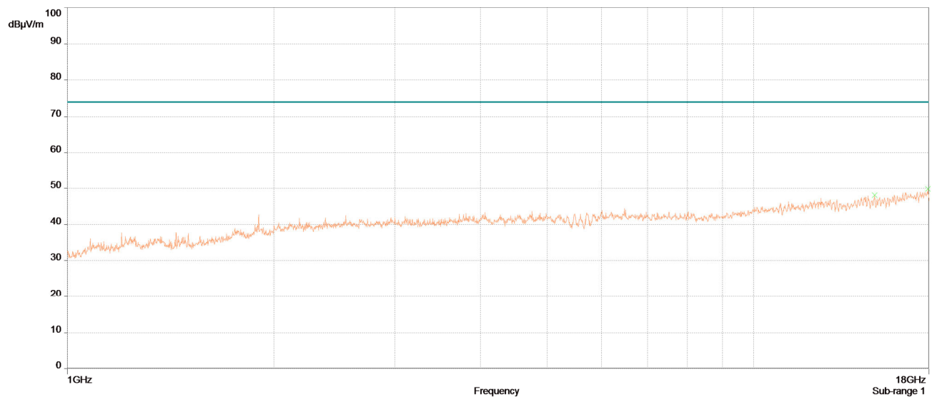
Radiated Spurious Emissions, 1GHz -18 GHz, BT Low Channel, Peak (Worst Case Pol)
