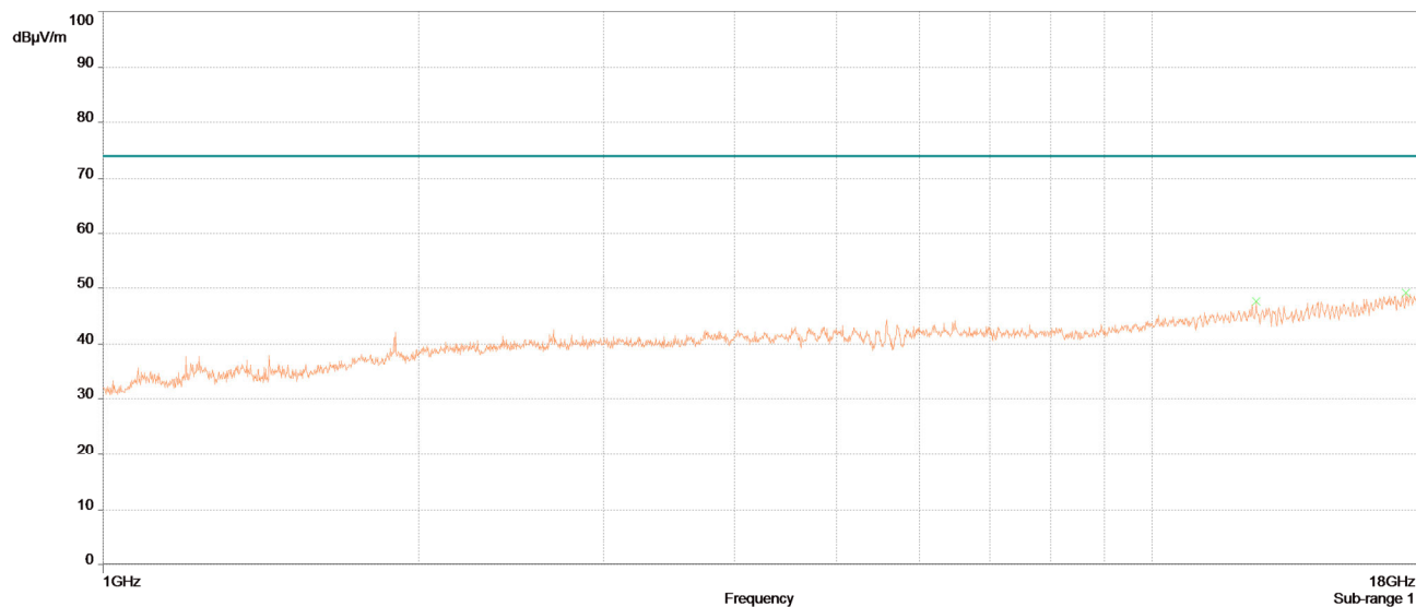
Radiated Spurious Emissions, 1GHz -18 GHz, BLE Mid Channel, Peak (Worst Case Pol)
