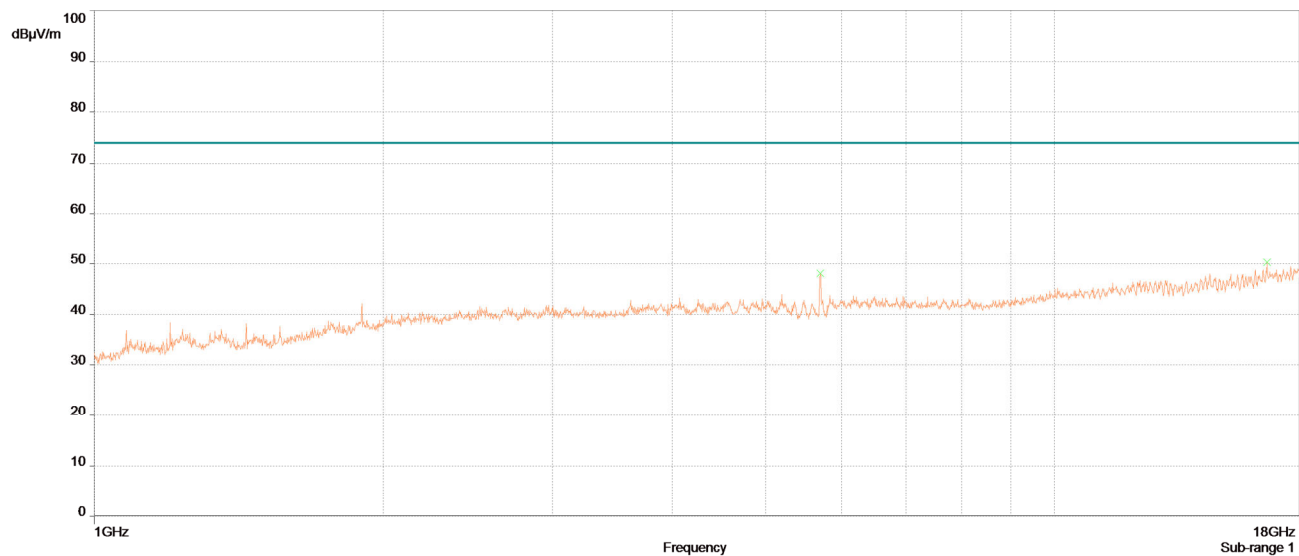
Radiated Spurious Emissions, 1GHz -18 GHz, BLE High Channel, Peak (Worst Case Pol)
