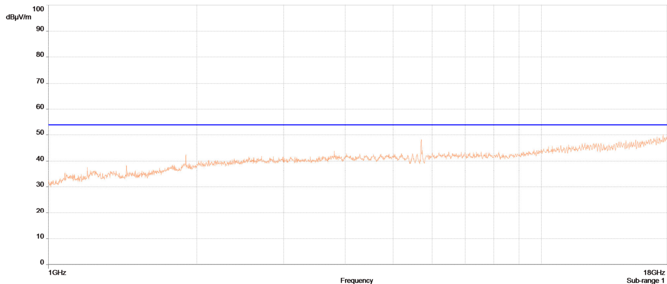
Radiated Spurious Emissions, 1GHz -18 GHz, BLE High Channel, Average (Worst Case Pol)
