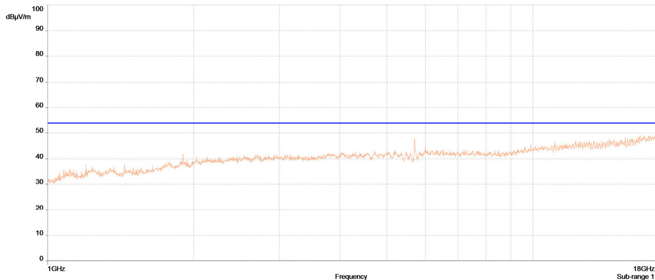
Radiated Spurious Emissions, 1GHz -18 GHz, BT High Channel, Average (Worst Case Pol)
