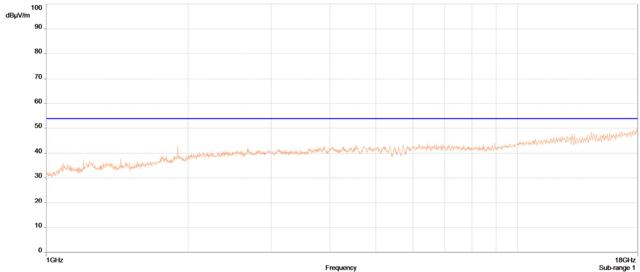
Radiated Spurious Emissions, 1GHz -18 GHz, BT Low Channel, Average (Worst Case Pol)
