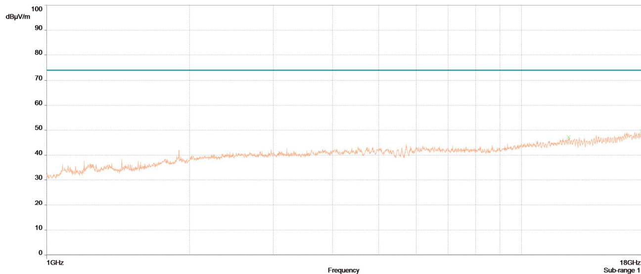
Radiated Spurious Emissions, 1GHz -18 GHz, BLE Low Channel, Peak (Worst Case Pol)
