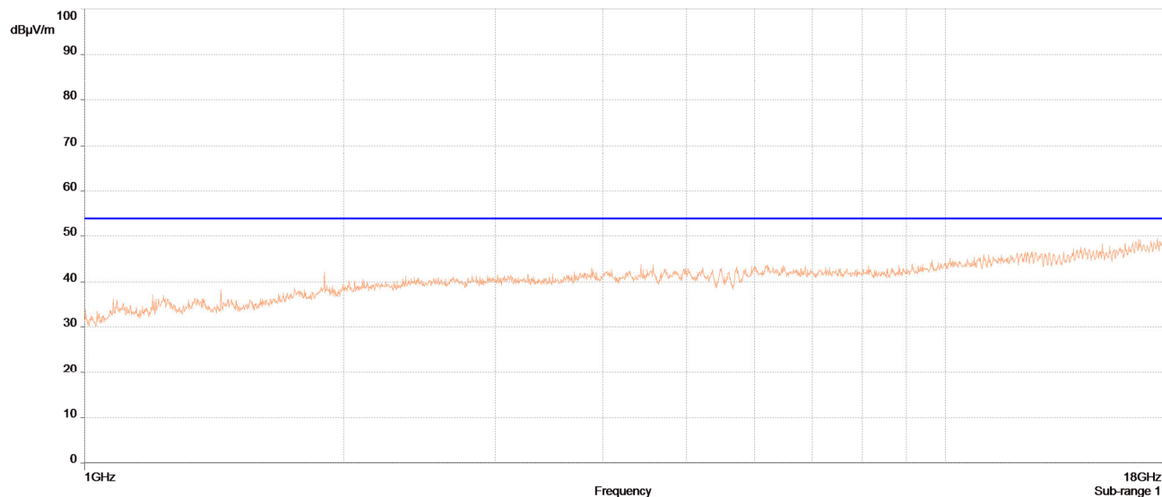
Radiated Spurious Emissions, 1GHz -18 GHz, BLE Low Channel, Average (Worst Case Pol)
