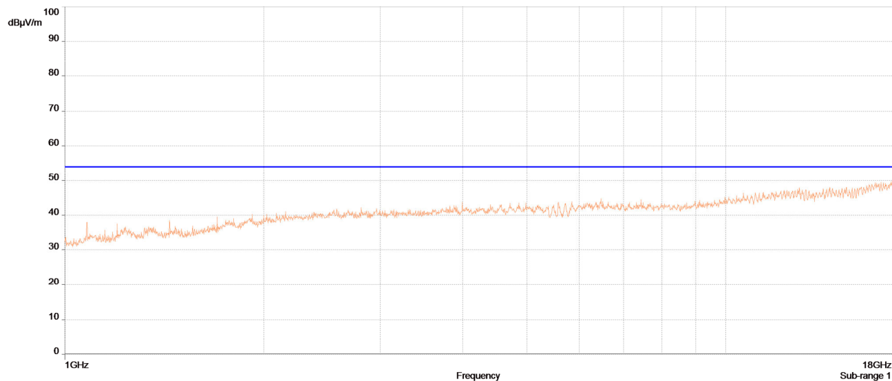
Radiated Spurious Emissions, 1GHz -18 GHz, BLE Mid Channel, Average (Worst Case Pol)
