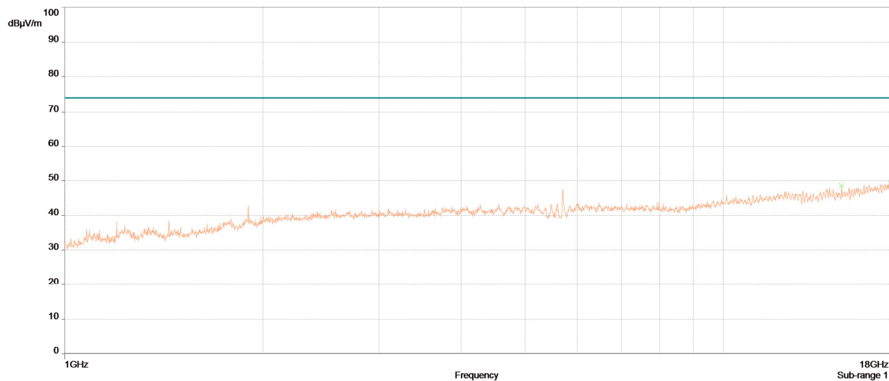
Radiated Spurious Emissions, 1GHz -18 GHz, BT High Channel, Peak (Worst Case Pol)
