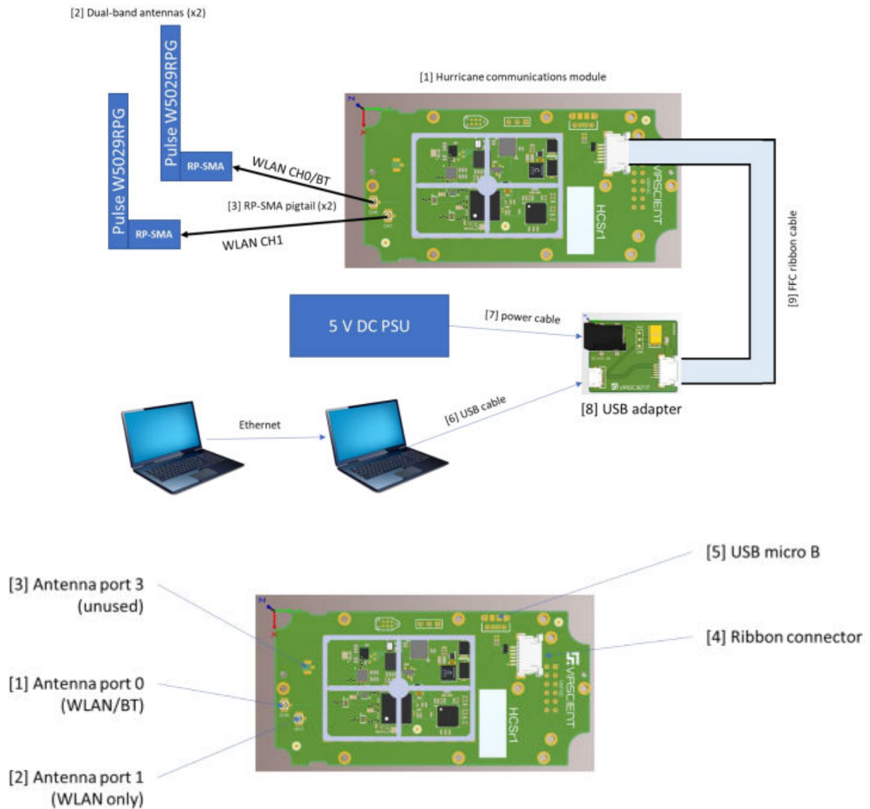
Block Diagram
