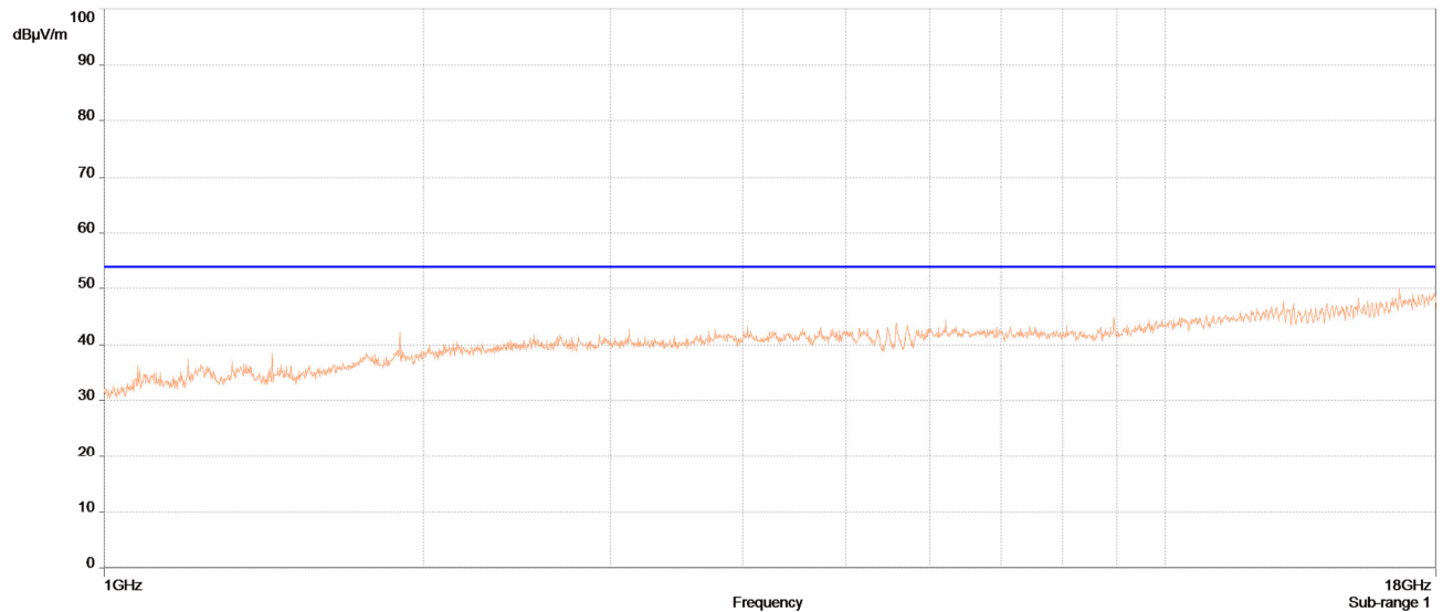
Radiated Spurious Emissions, 1GHz -18 GHz, BT Mid Channel, Average (Worst Case Pol)
